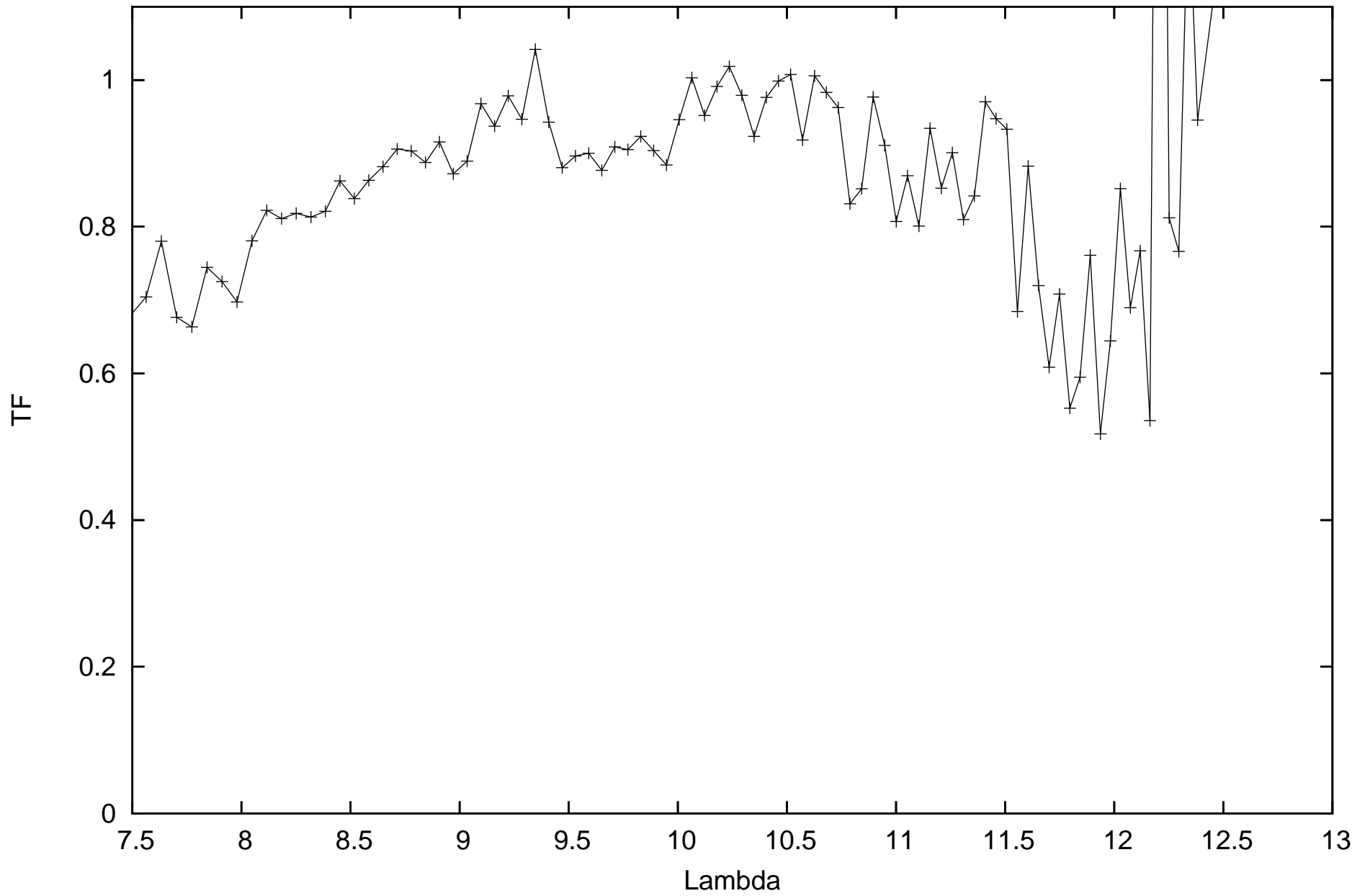
calHD112142_flux-0.18_diam5.44_r.MIDI.2012-01-24T08_22_22.969_C1A1
