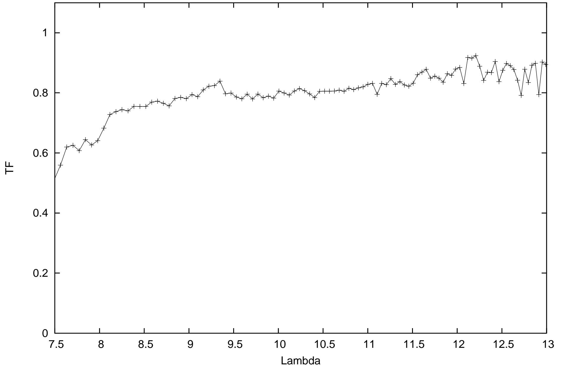
calHD120323_flux-2.02_diam13.25_r.MIDI.2012-06-25T01_24_53.969_C1A1
