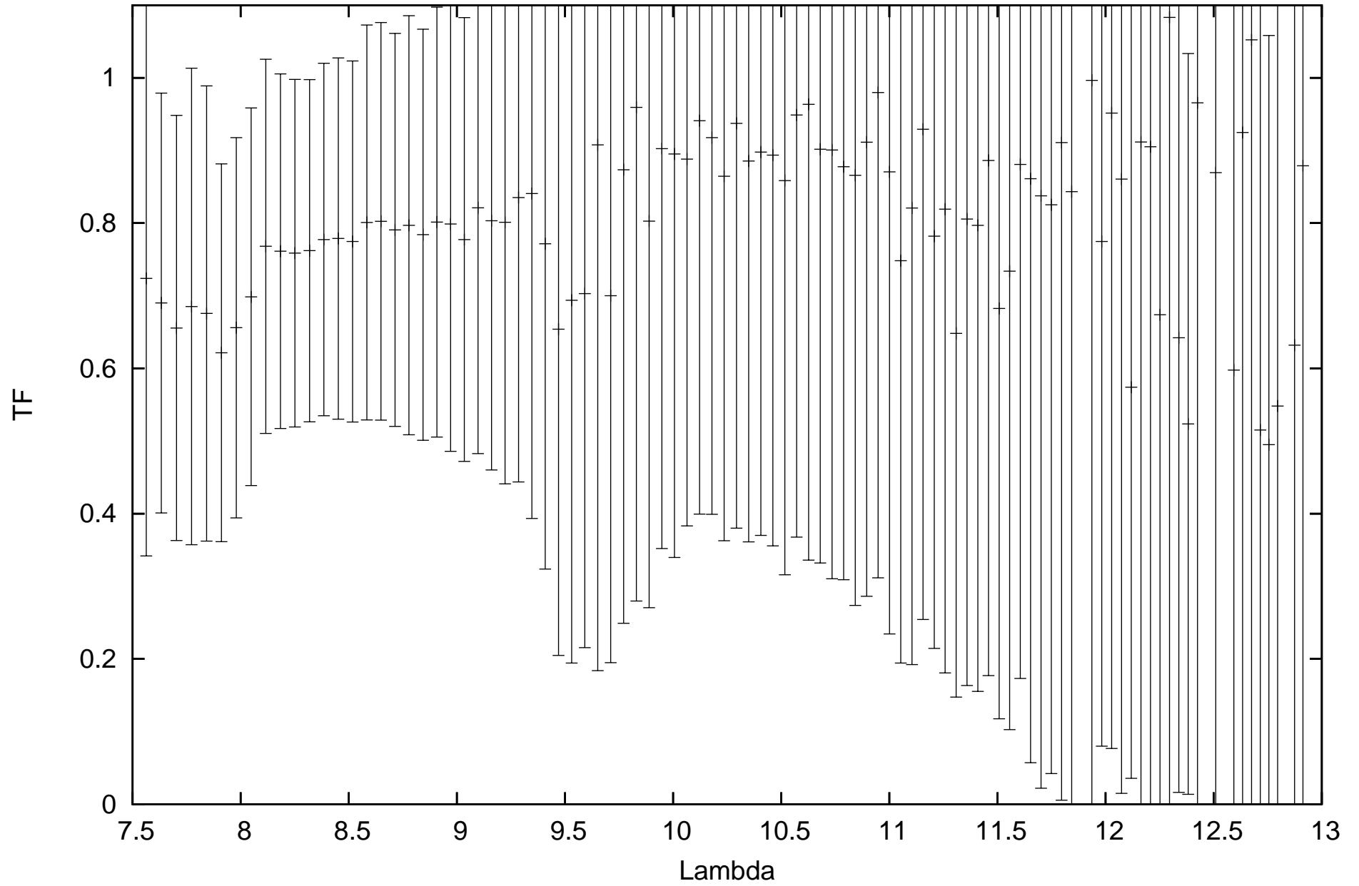
calHD123139_flux-0.39_diam5.34_r.MIDI.2012-05-01T04_13_47.293_B2A1
