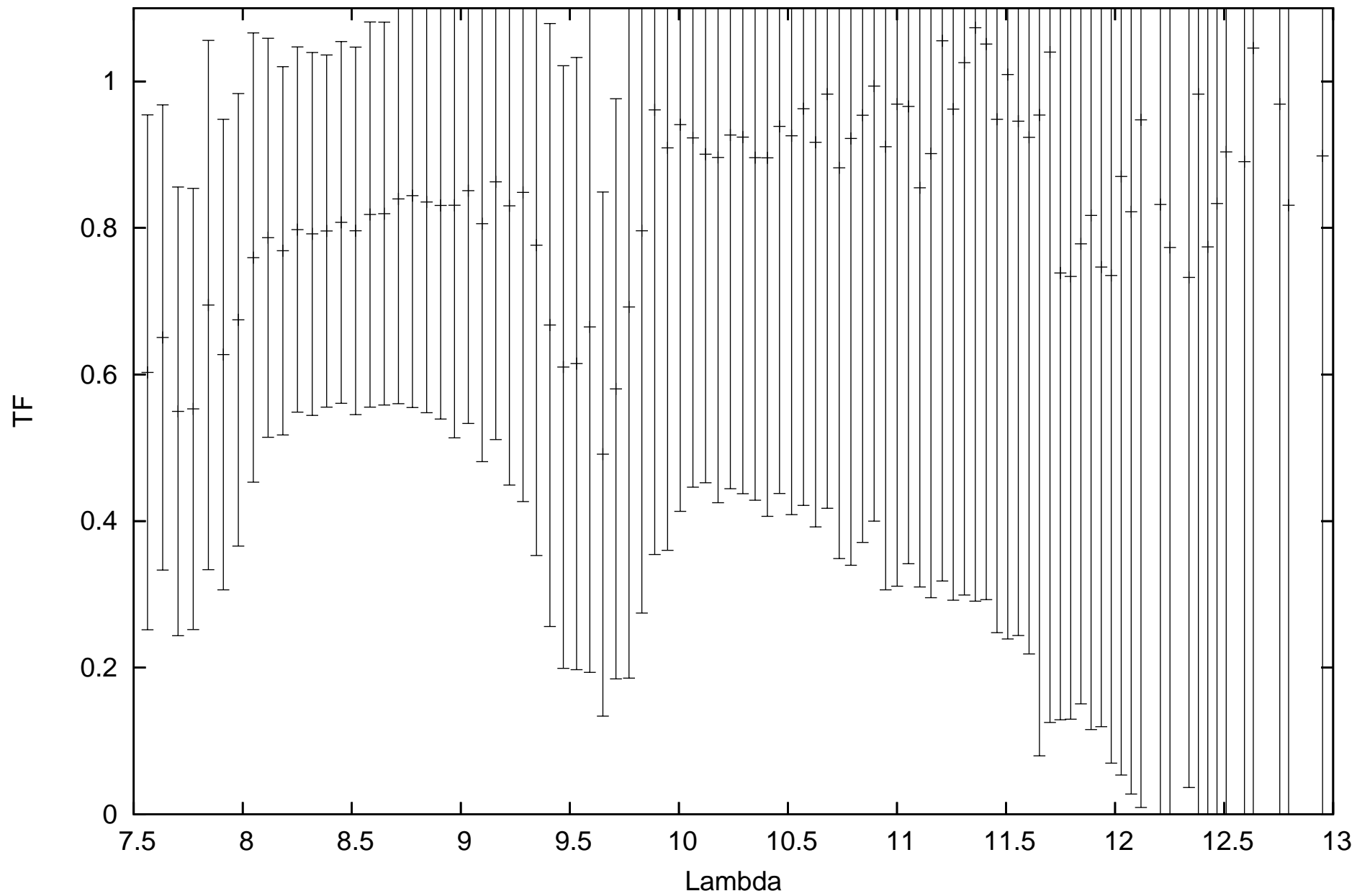
calHD123139_flux-0.39_diam5.34_r.MIDI.2012-05-02T00_35_33.293_C1B2
