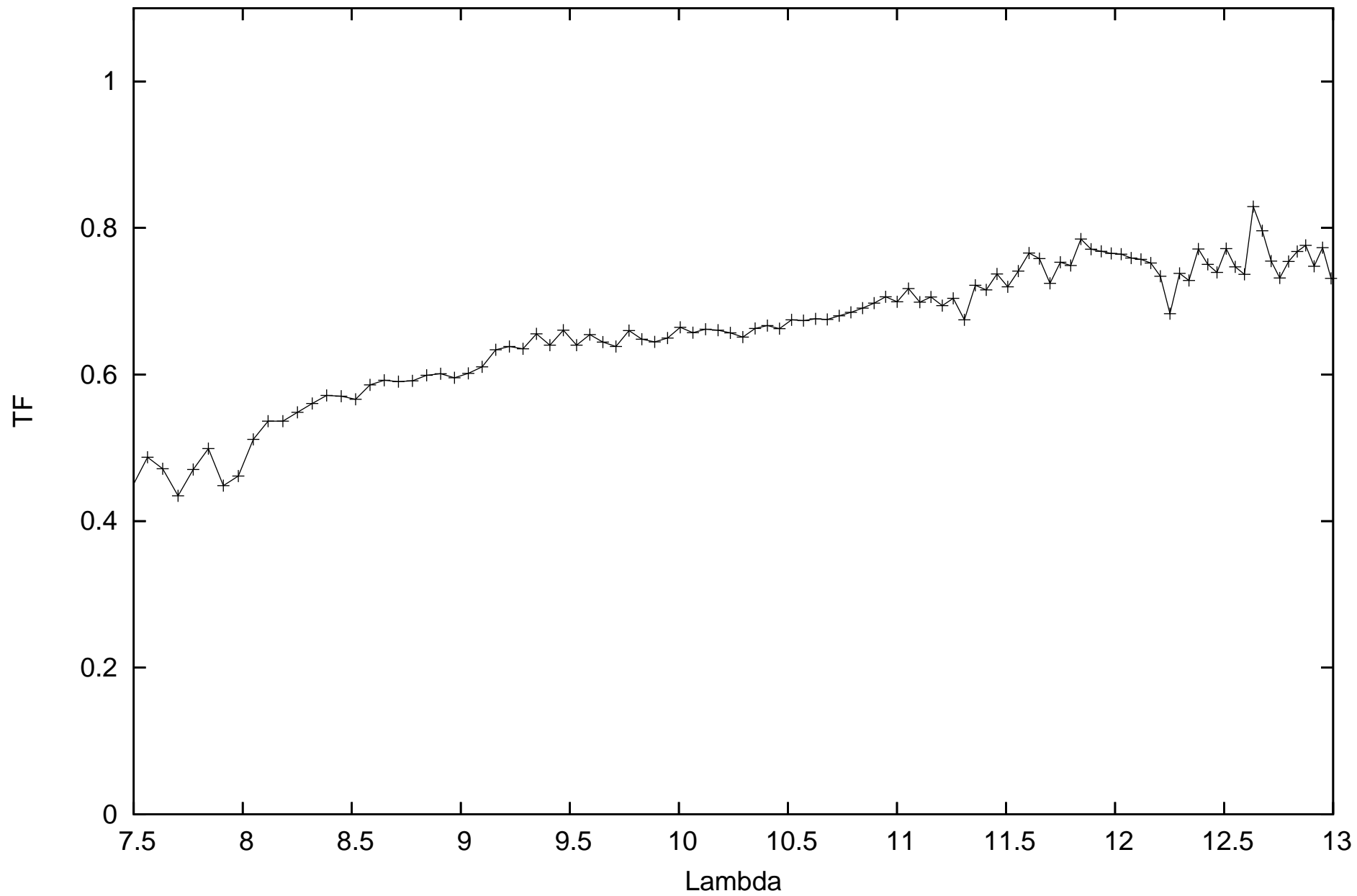
calHD152980_flux0.64_diam3.62_r.MIDI.2012-04-05T08_32_21.969_U2U3
