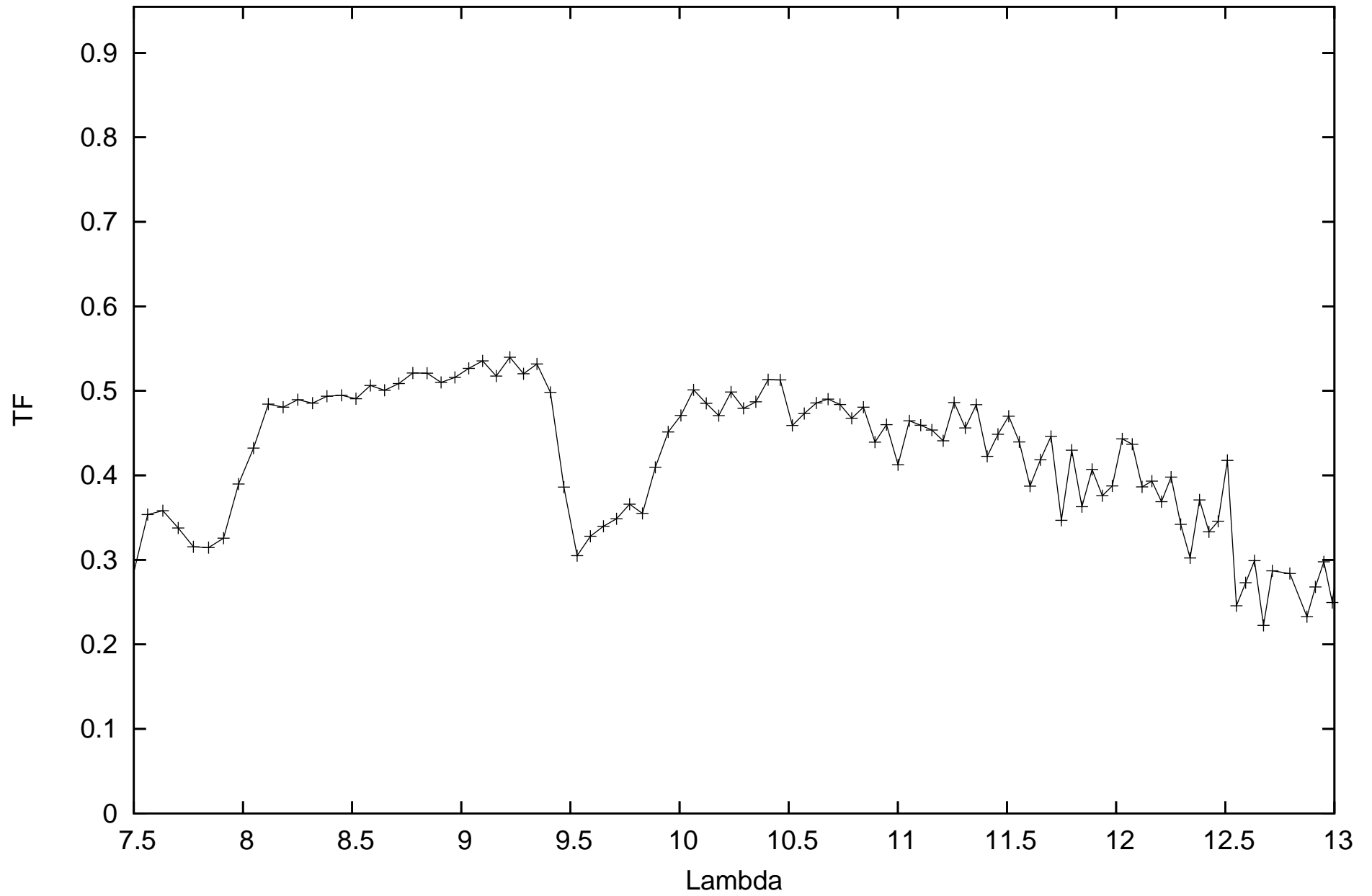
calHD167618_flux-1.82_diam11.66_r.MIDI.2012-06-08T08_47_52.970_K0I1
