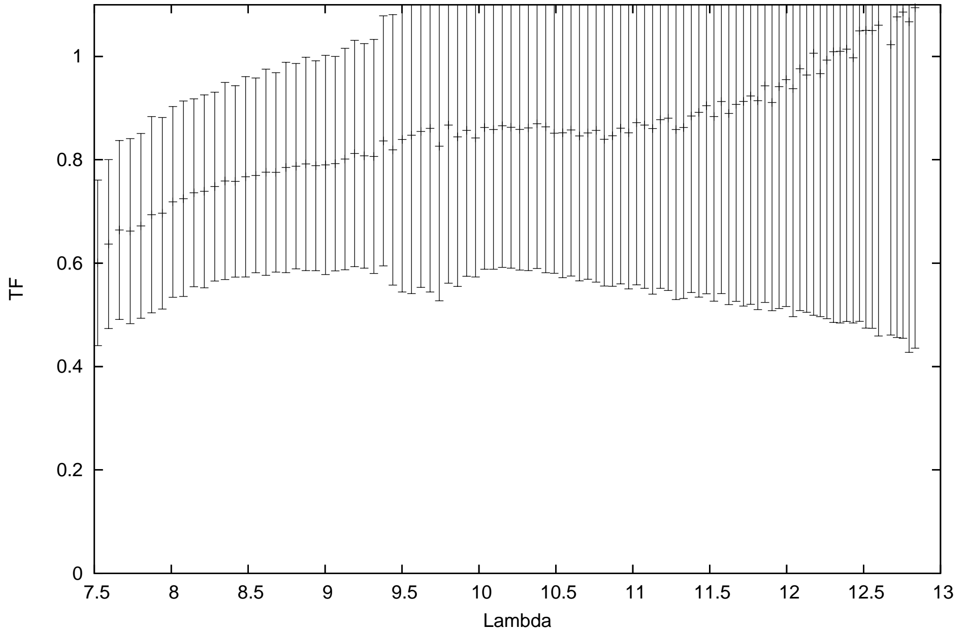
calHD167618_flux-1.82_diam11.66_r.MIDI.2012-07-22T01_10_05.000_D0A1
