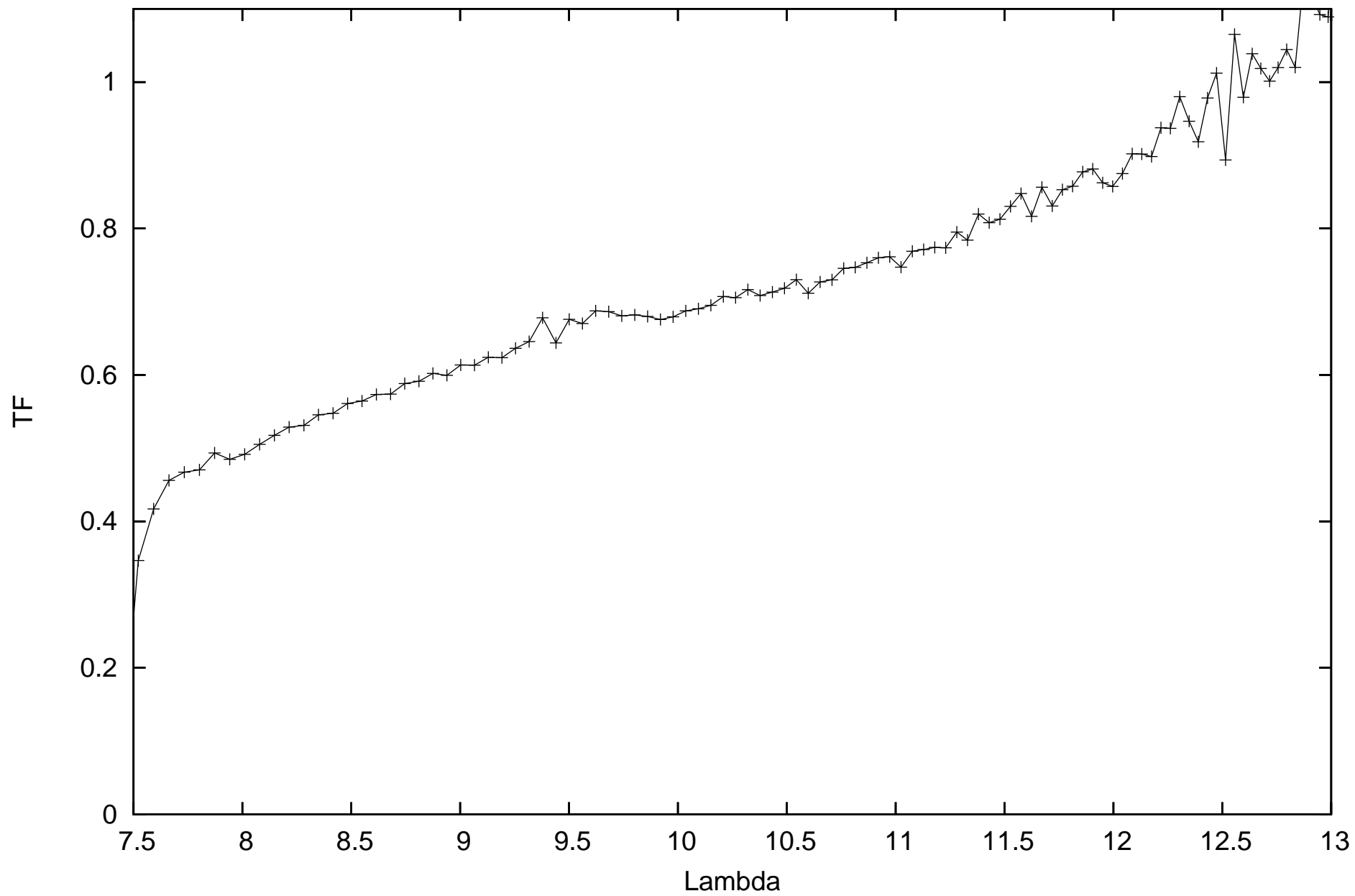
calHD167618_flux-1.82_diam11.66_r.MIDI.2012-09-02T01_48_57.000_K0G1
