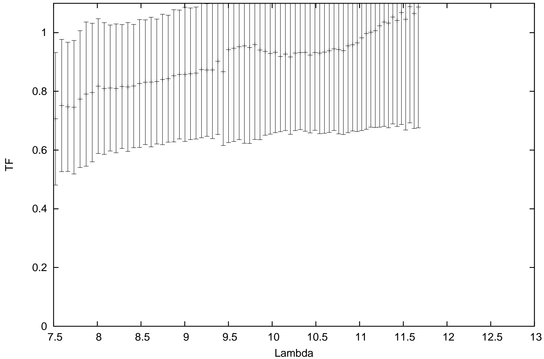
calHD167618_flux-1.82_diam11.66_r.MIDI.2012-09-22T02_42_05.000_C1B2
