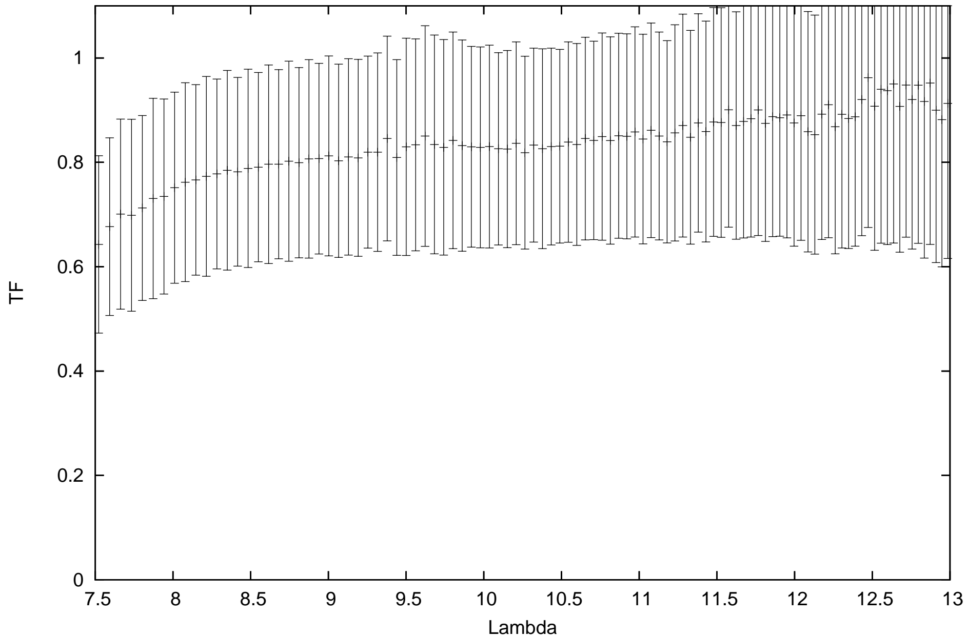
calHD167618_flux-1.82_diam11.66_r.MIDI.2012-09-26T01_05_21.000_C1A1
