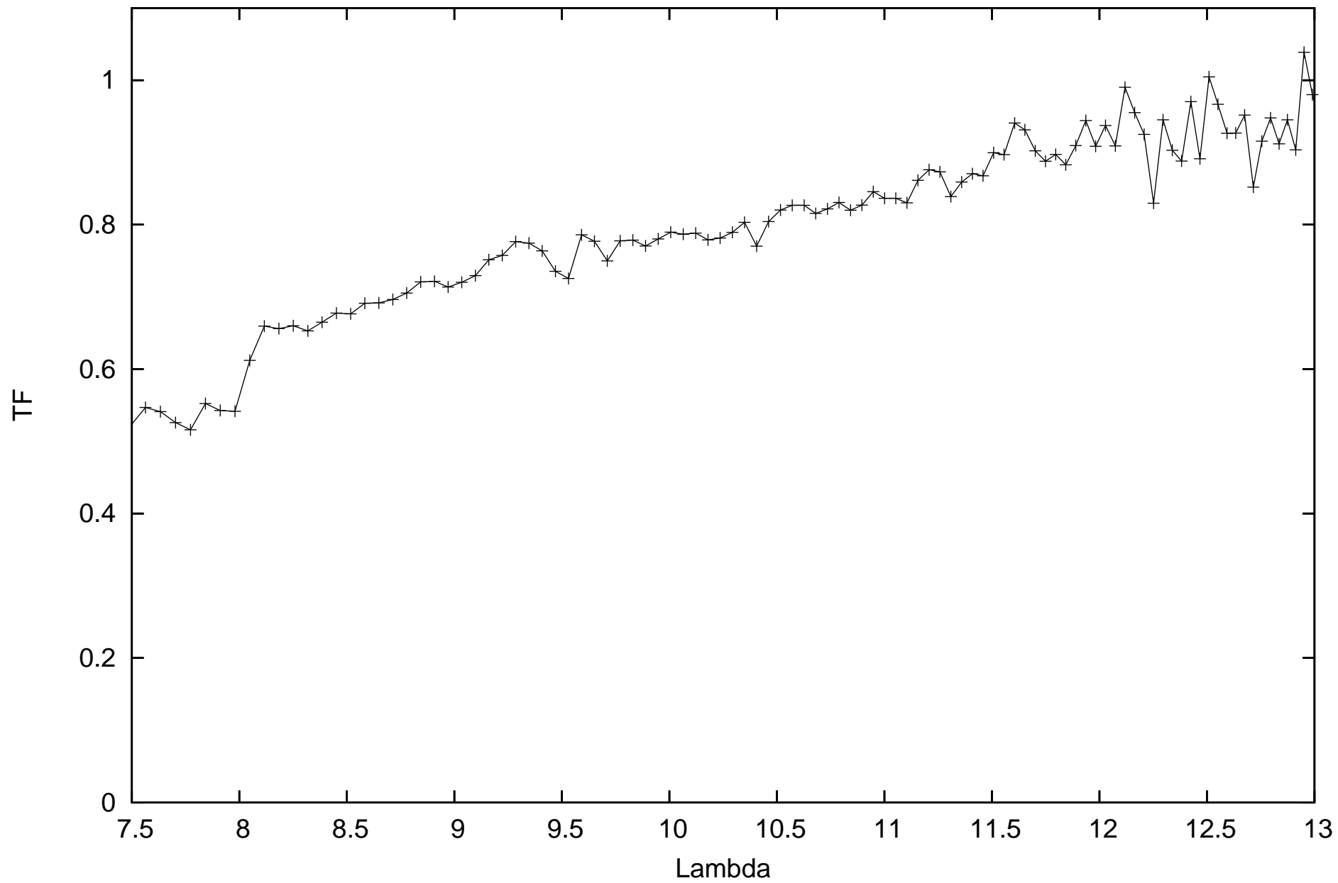
calHD167618_flux-1.82_diam11.66_r.MIDI.2012-09-27T00_03_20.113_B2A1
