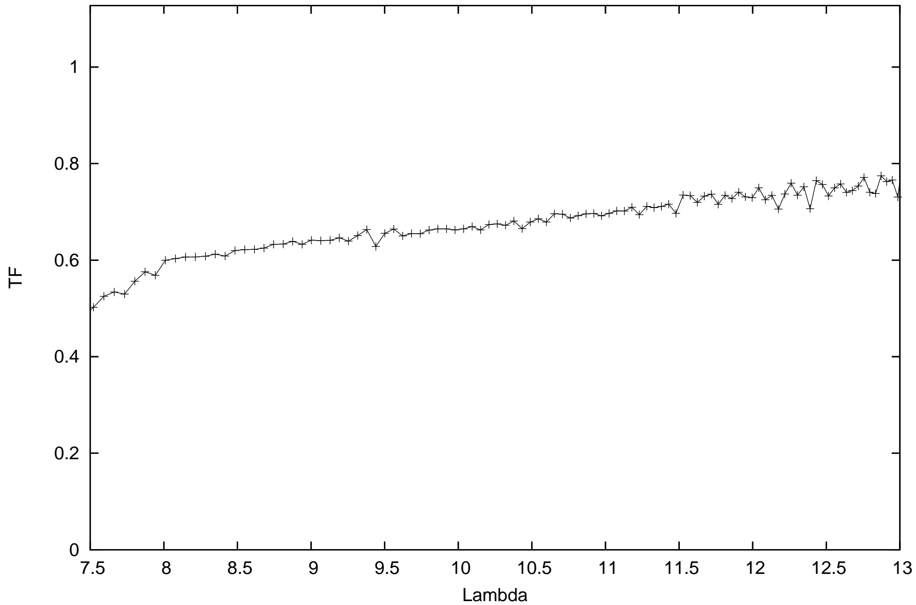
calHD167618_flux-1.82_diam11.66_r.MIDI.2012-10-20T00_09_01.000_C1A1
