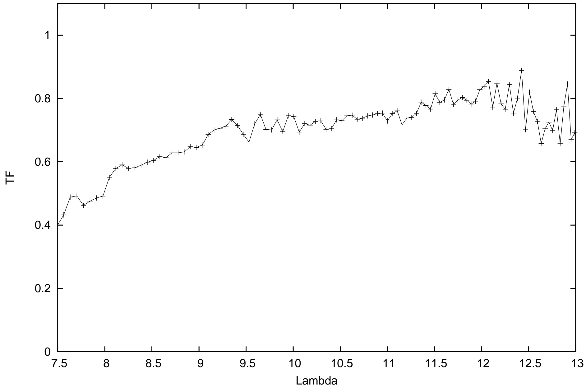
calHD206778_flux-1.04_diam7.59_r.MIDI.2012-10-12T00_15_48.135_A1G1
