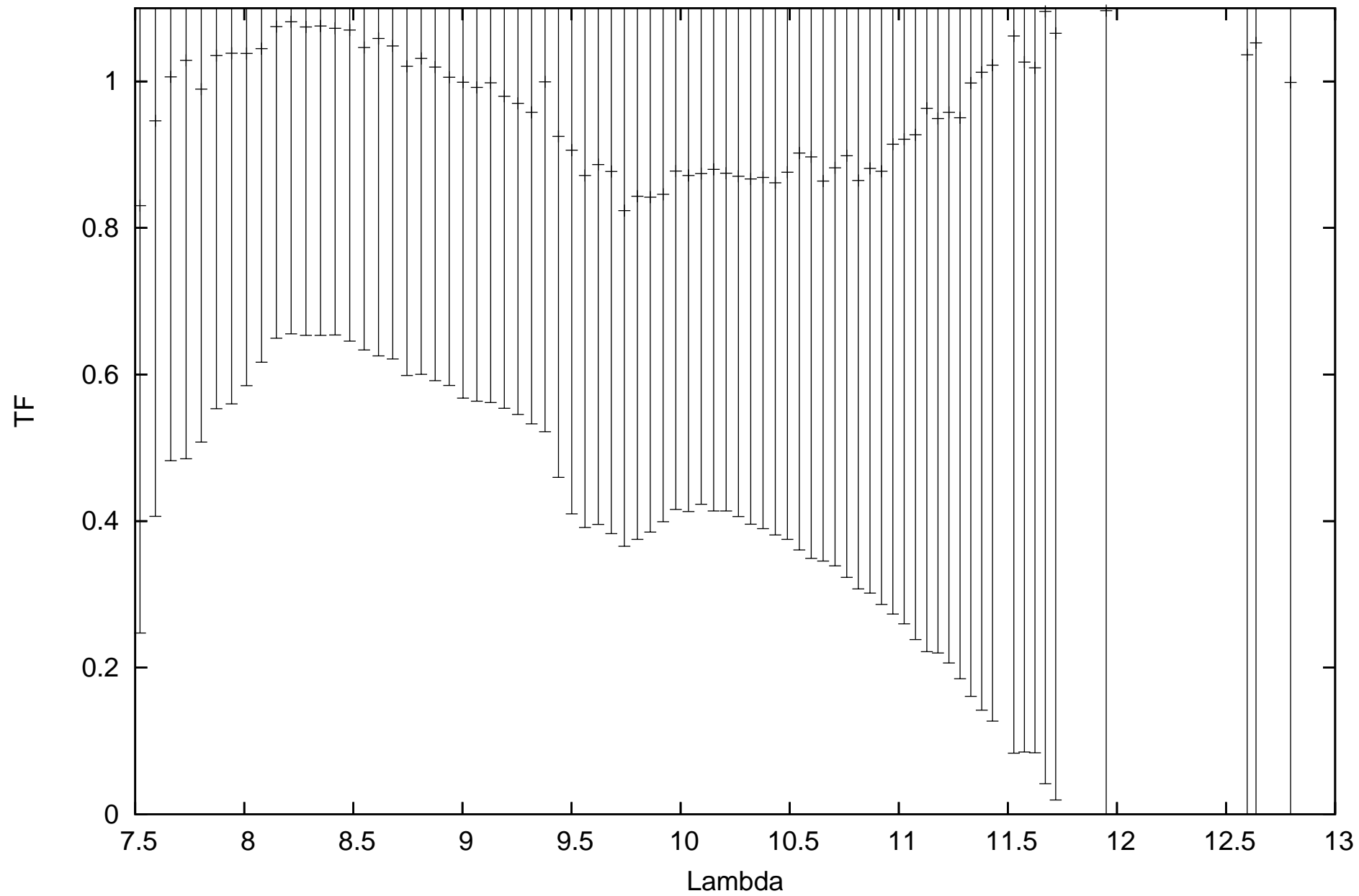
calHD48915_flux-1.39_diam6.09_r.MIDI.2012-01-09T04_50_27.000_G1A1
