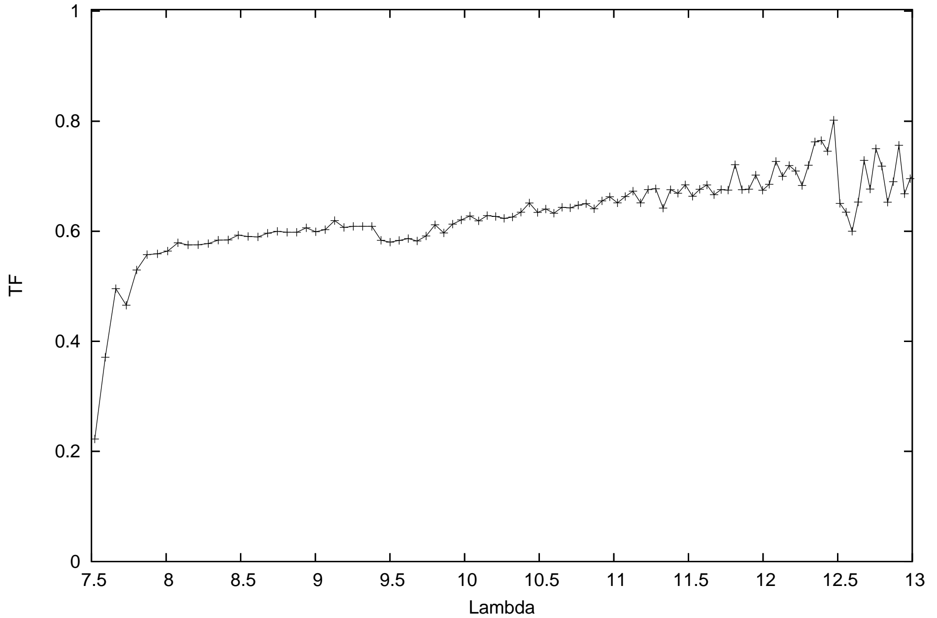
calHD48915_flux-1.39_diam6.09_r.MIDI.2012-03-27T01_00_21.000_G111
