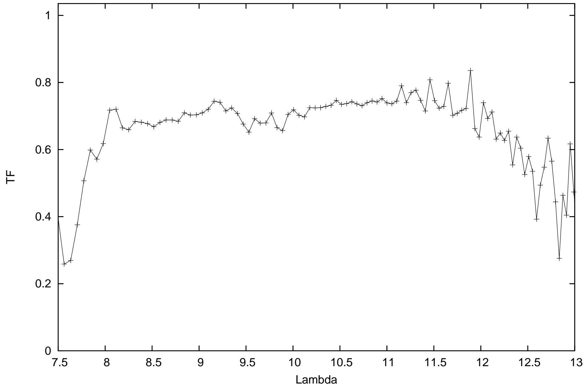
calHD48915_flux-1.39_diam6.09_r.MIDI.2012-03-27T01_09_00.113_G111
