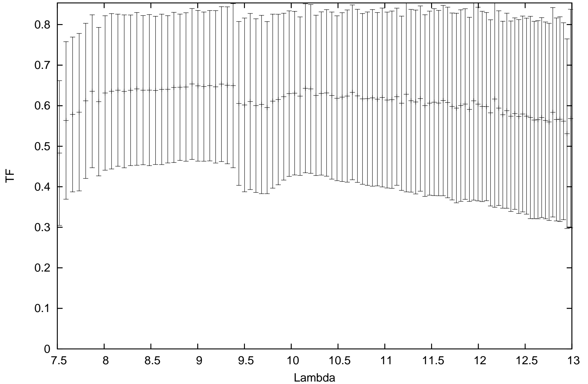
calHD63700_flux0.76_diam3.18_r.MIDI.2012-02-04T06_40_10.000_U3U4
