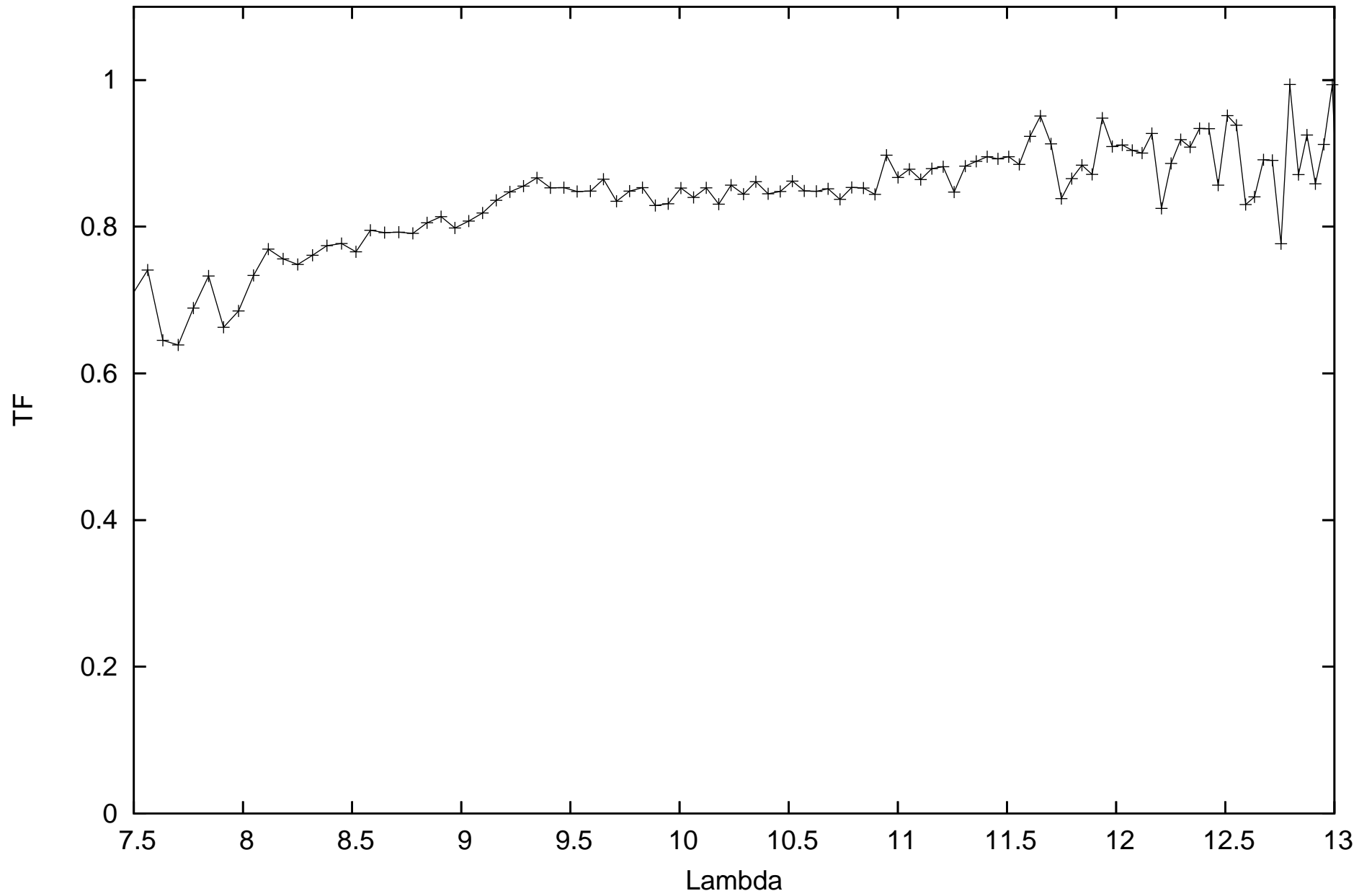
calHD81797_flux-1.49_diam9.14_r.MIDI.2012-01-24T04_29_13.970_C1A1
