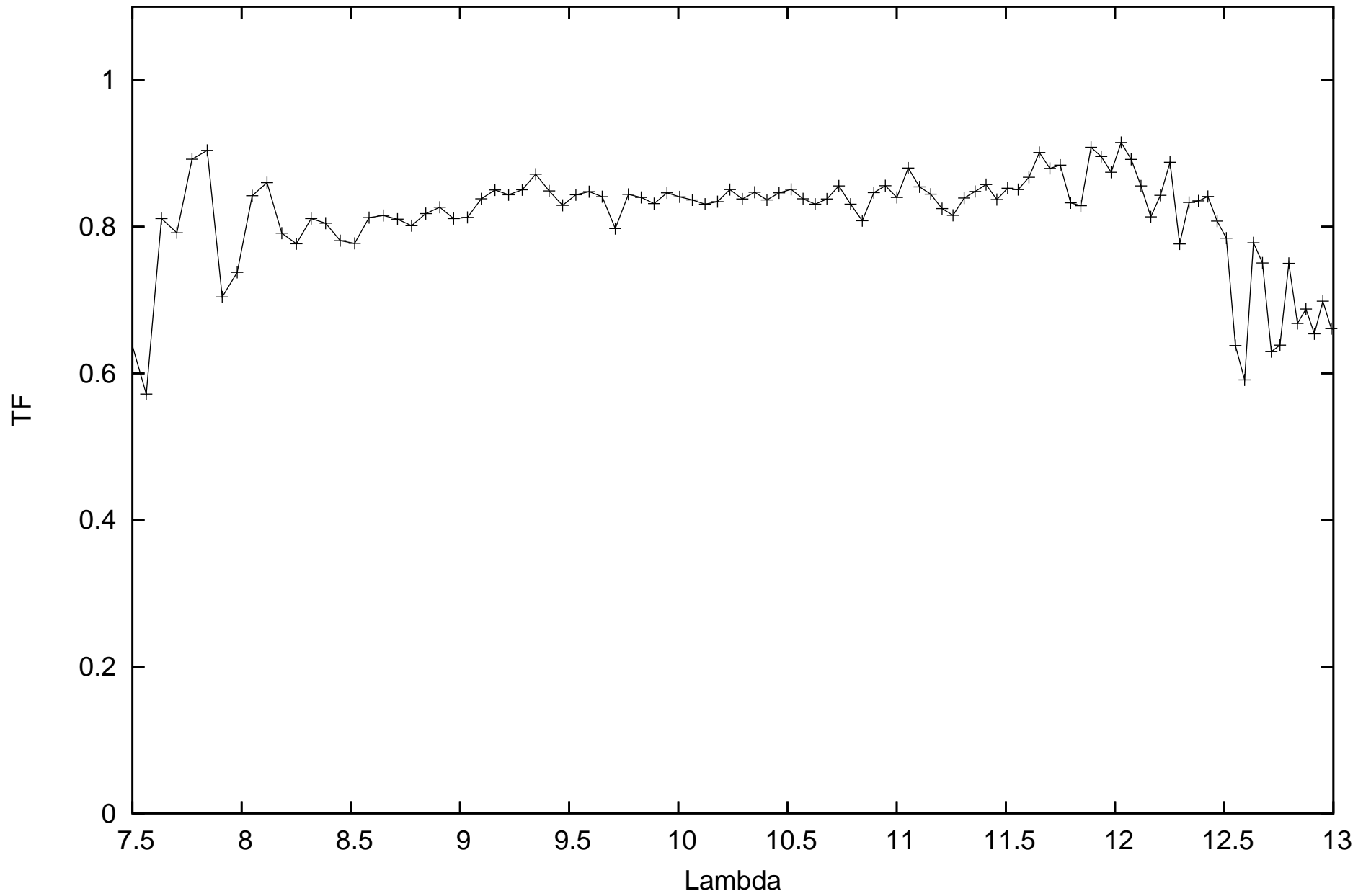
calHD81797_flux-1.49_diam9.14_r.MIDI.2012-01-28T07_45_26.970_C1B2
