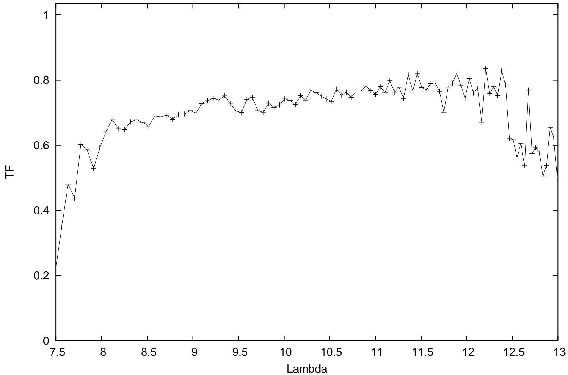
calHD81797_flux-1.49_diam9.14_r.MIDI.2012-02-01T07_40_45.970_B2A1
