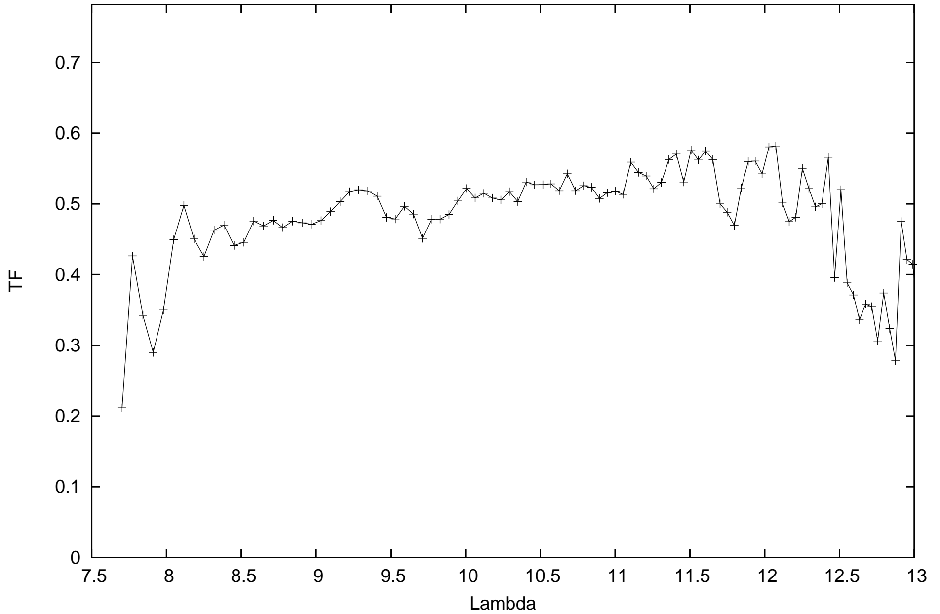
calHD81797_flux-1.49_diam9.14_r.MIDI.2012-02-12T07_15_40.293_C1A1
