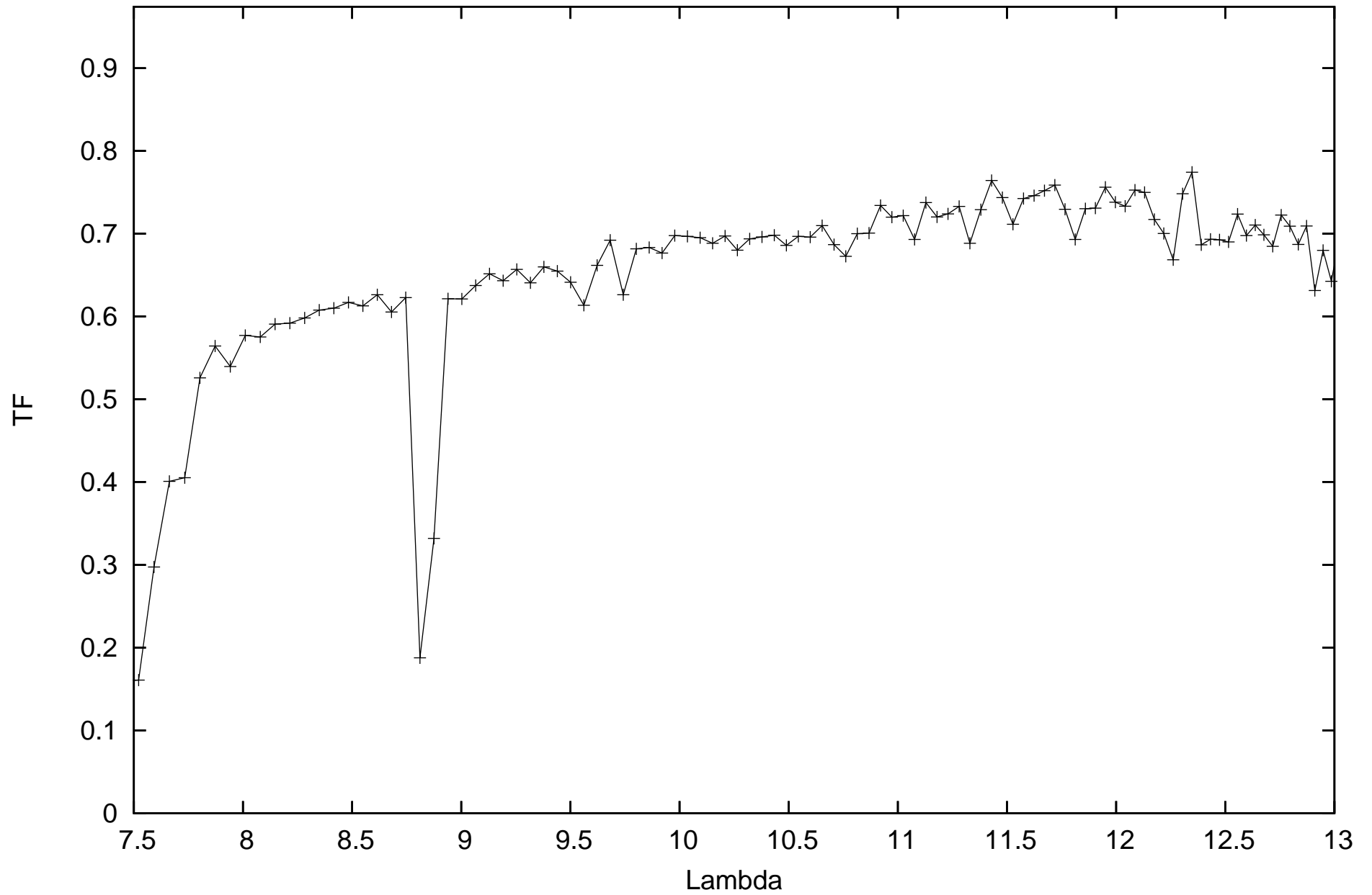
calHD81797_flux-1.49_diam9.14_r.MIDI.2012-04-02T04_29_34.000_G1A1
