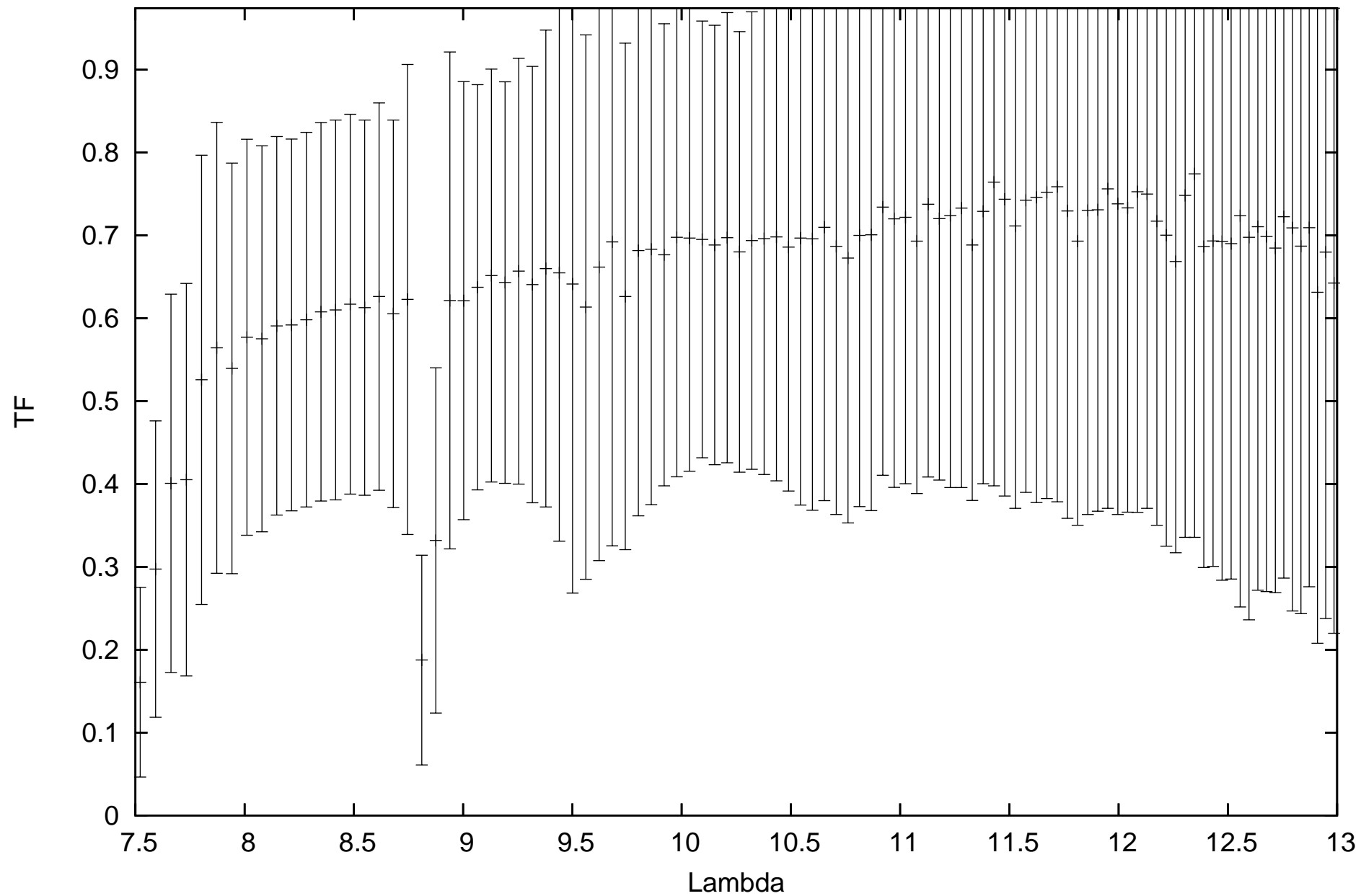
calHD81797_flux-1.49_diam9.14_r.MIDI.2012-04-02T04_29_34.000_G1A1
