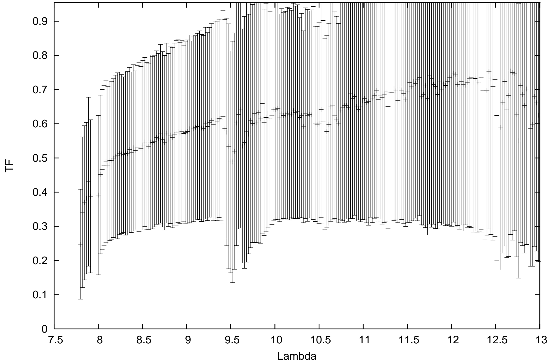
calHIP19038_flux1.83316_diam1.9_r.MIDI.2012-11-02T06_55_15.000_U2U4
