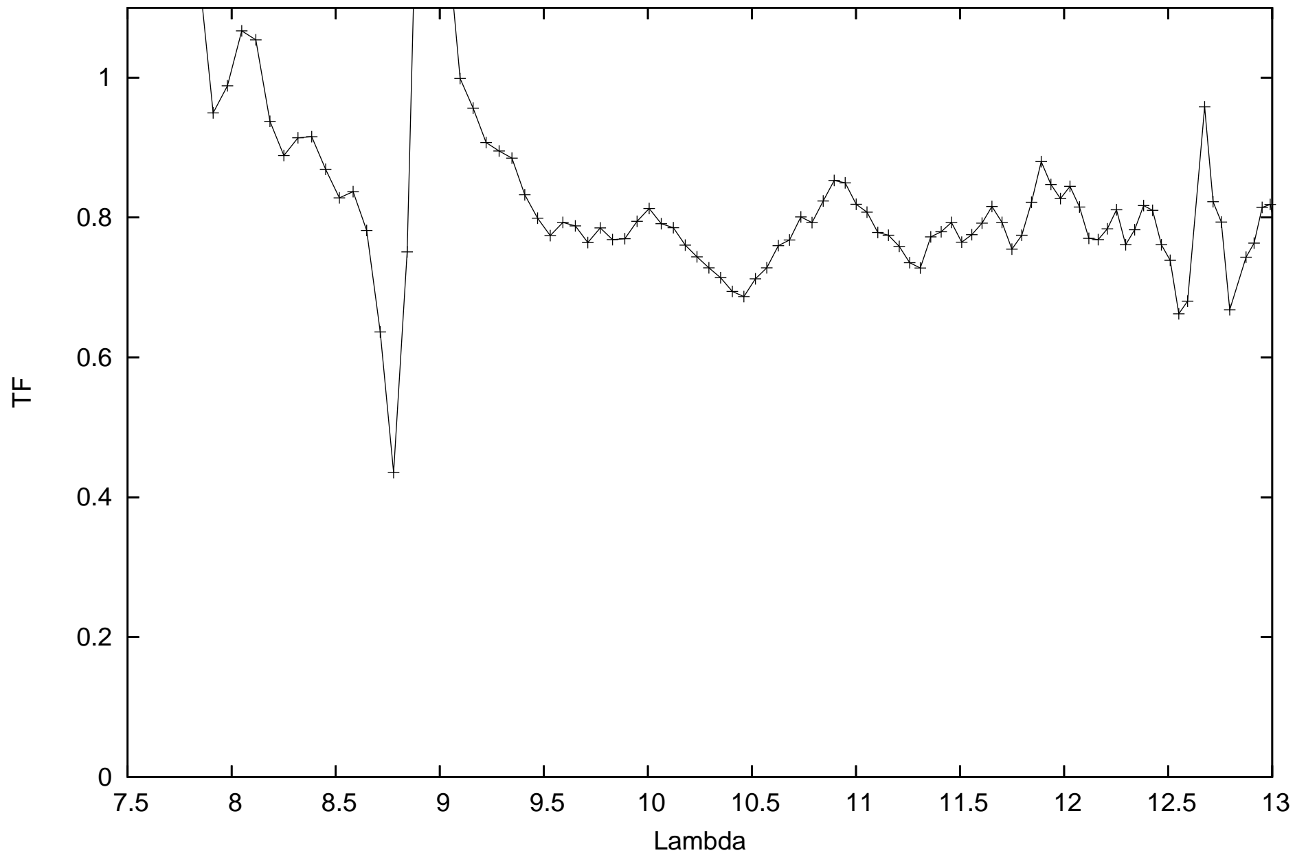
calHIP21421_flux-3.13927_diam20.4_r.MIDI.2012-02-18T01_12_47.112_C1A1
