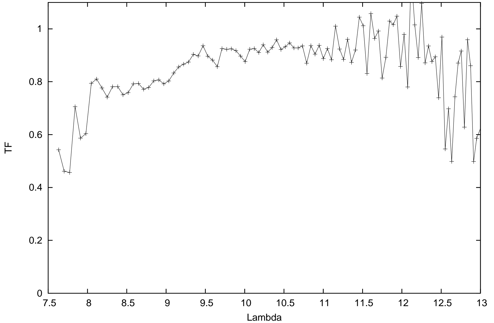
calHIP46701_flux-0.68631_diam6.952948_r.MIDI.2012-02-12T03_59_40.933_D0B2
