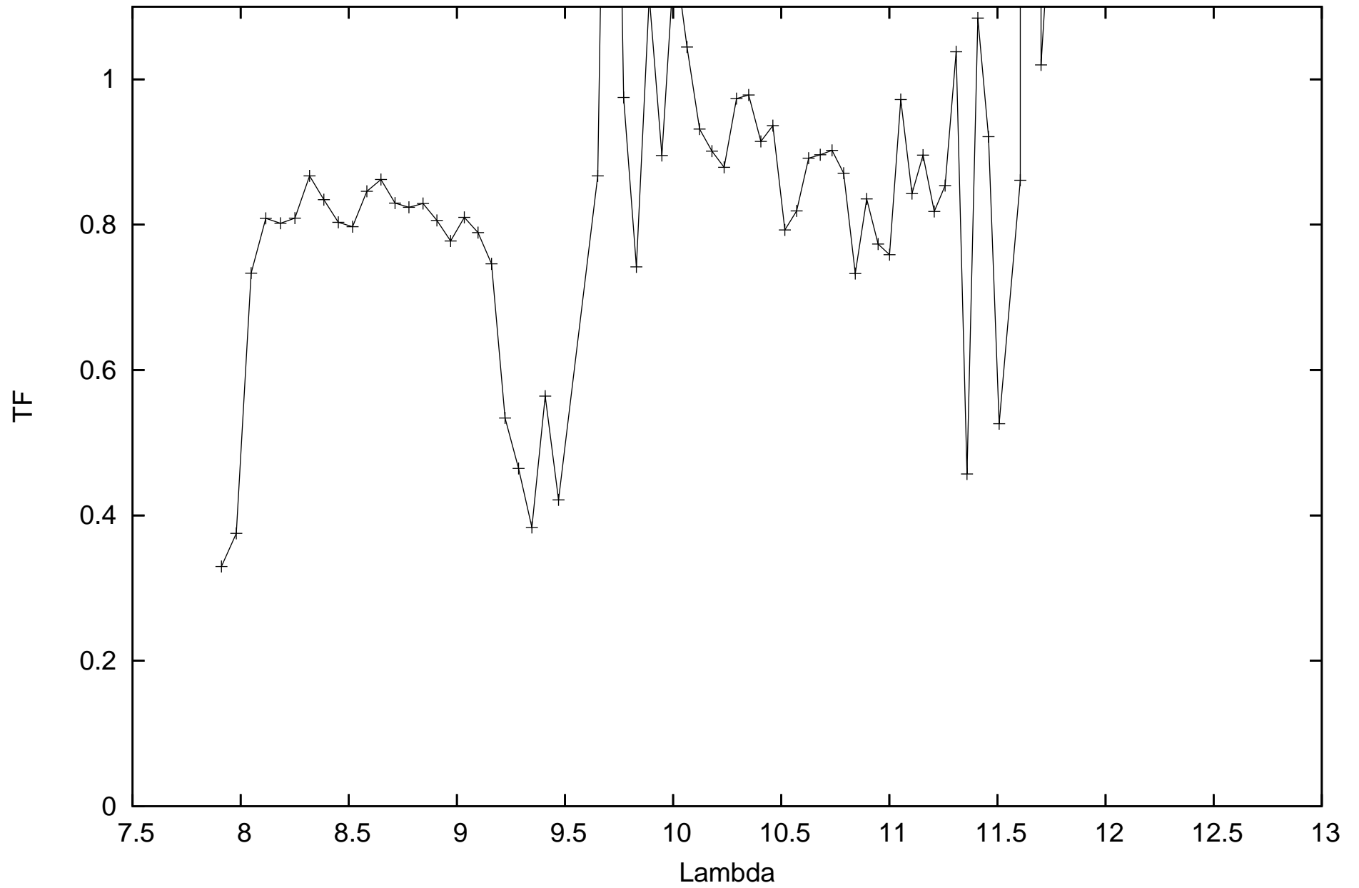
calHIP50371_flux-0.22962_diam5.18_r.MIDI.2012-01-29T01_59_05.969_D0B2
