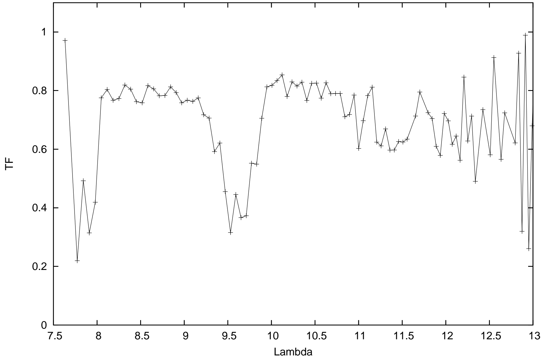
calHIP50371_flux-0.22962_diam5.18_r.MIDI.2012-01-29T05_30_36.932_D0B2
