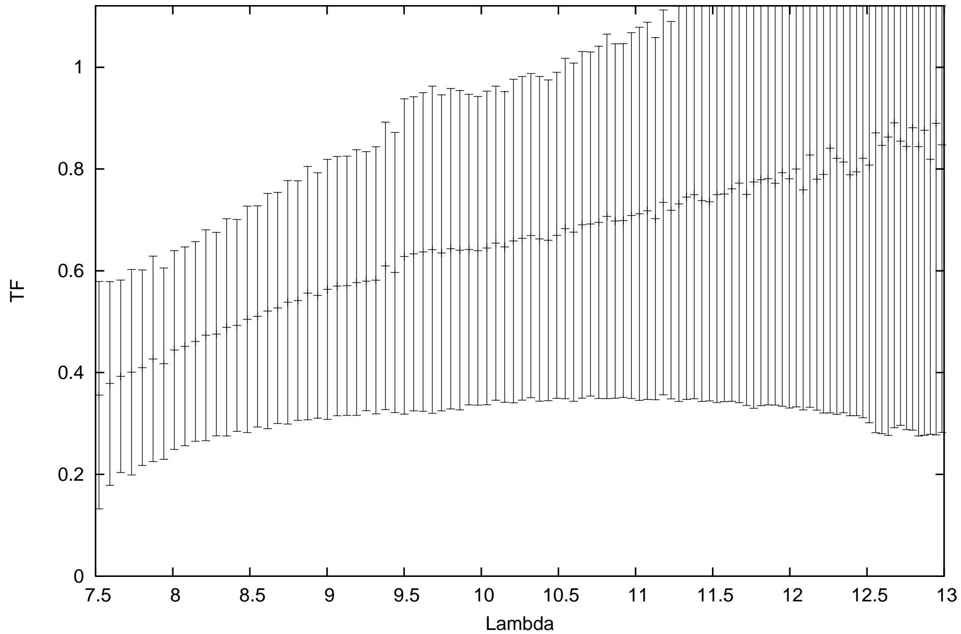
calHIP73714_flux-1.78451_diam11.15_r.MIDI.2012-05-27T04_44_07.000_K0G1
