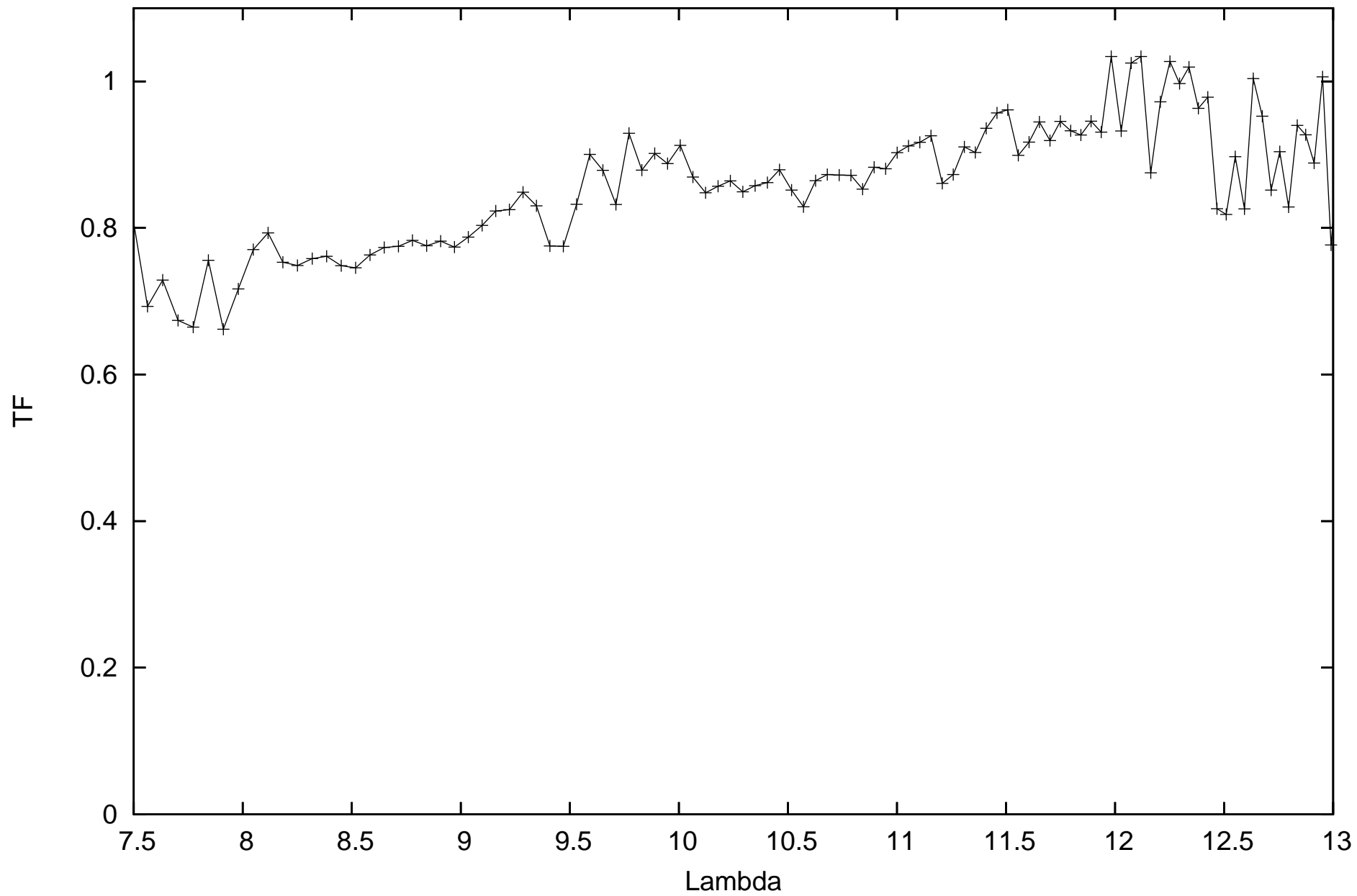
calHIP82273_flux-1.42243_diam8.91_r.MIDI.2012-01-25T08_08_26.970_C1A1
