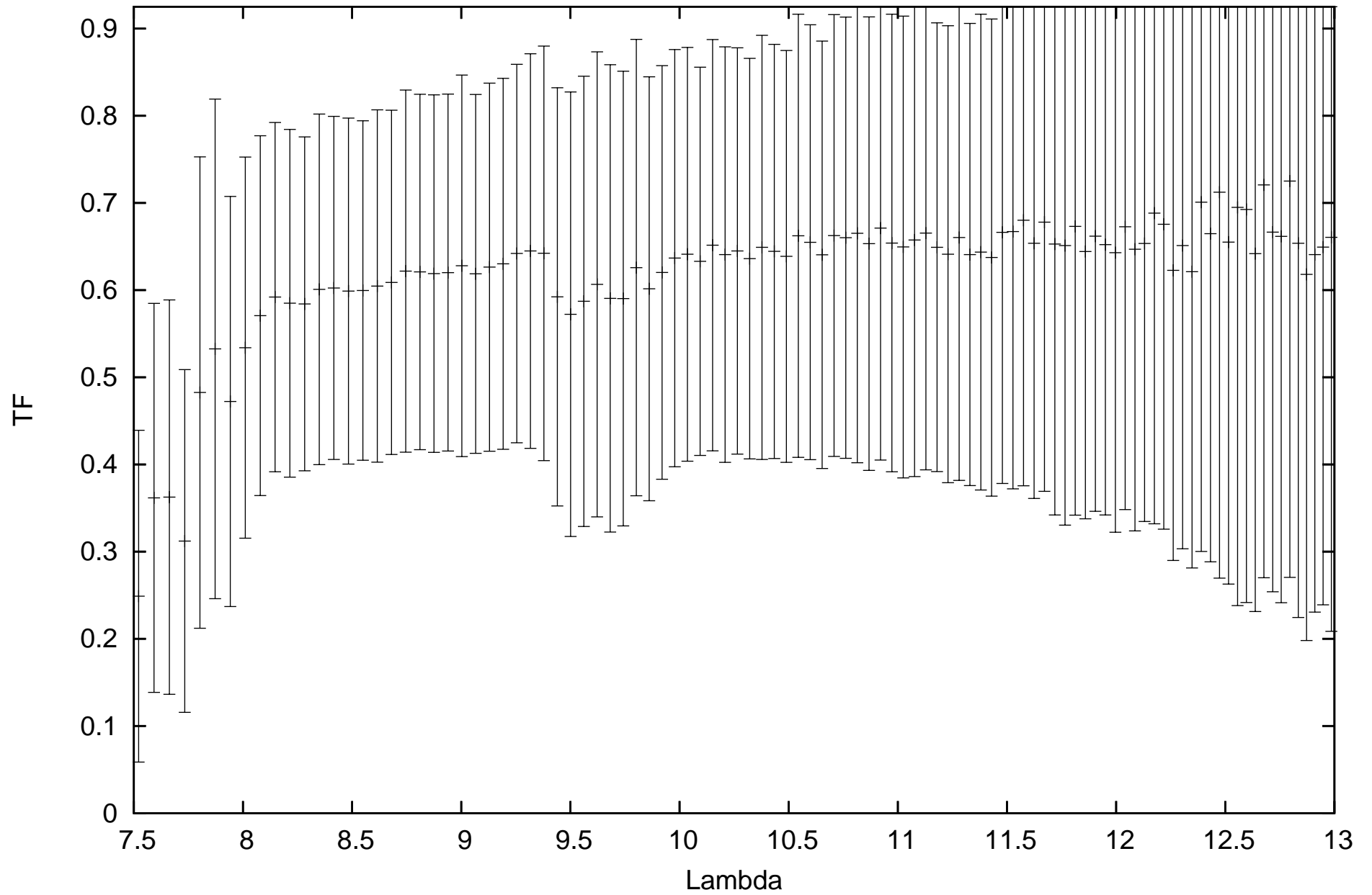
calHIP82273_flux-1.42243_diam8.91_r.MIDI.2012-03-26T09_25_40.000_K011
