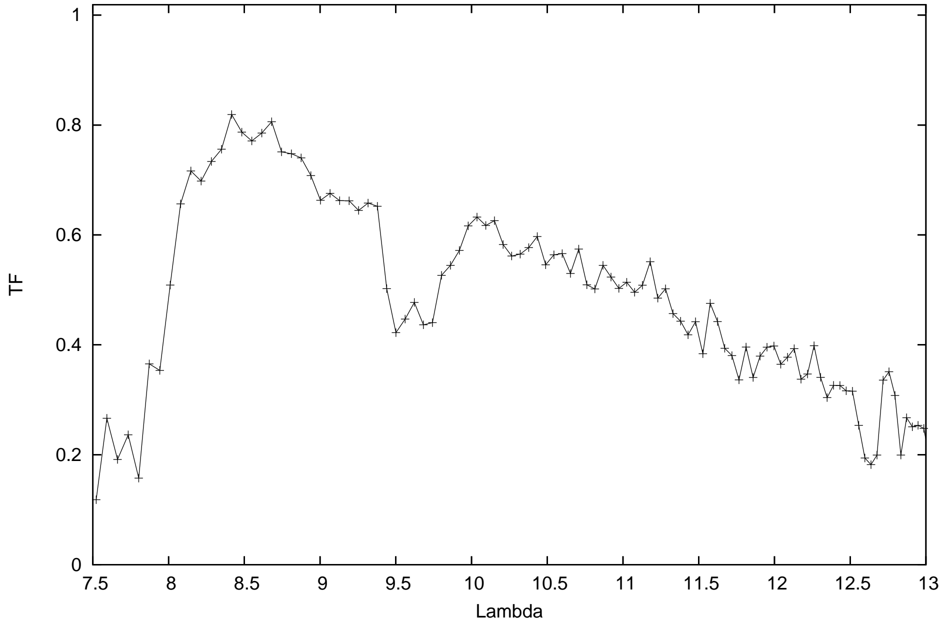
calHIP82363_flux-0.3207_diam5.52_r.MIDI.2012-03-26T08_39_21.000_K0I1
