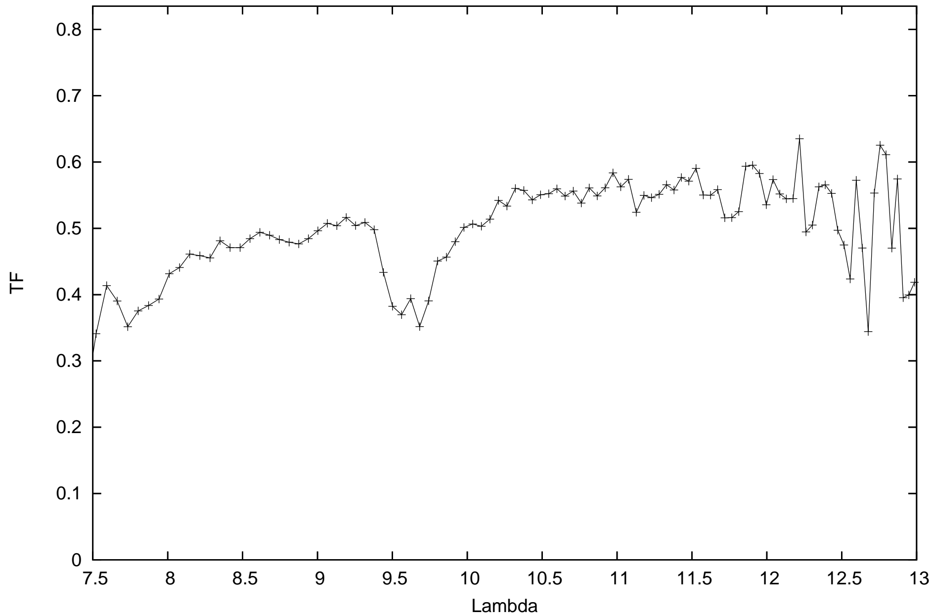
calHIP82363_flux-0.3207_diam5.52_r.MIDI.2012-10-20T00_36_45.000_C1A1
