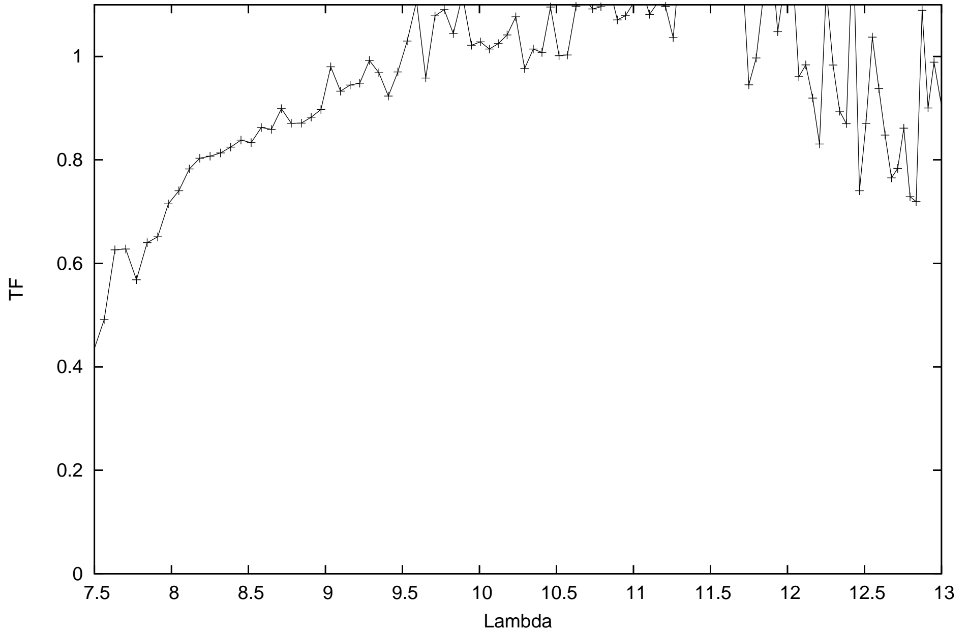
calHIP89931_flux-0.511_diam5.87_r.MIDI.2012-07-01T08_09_49.135_K011
