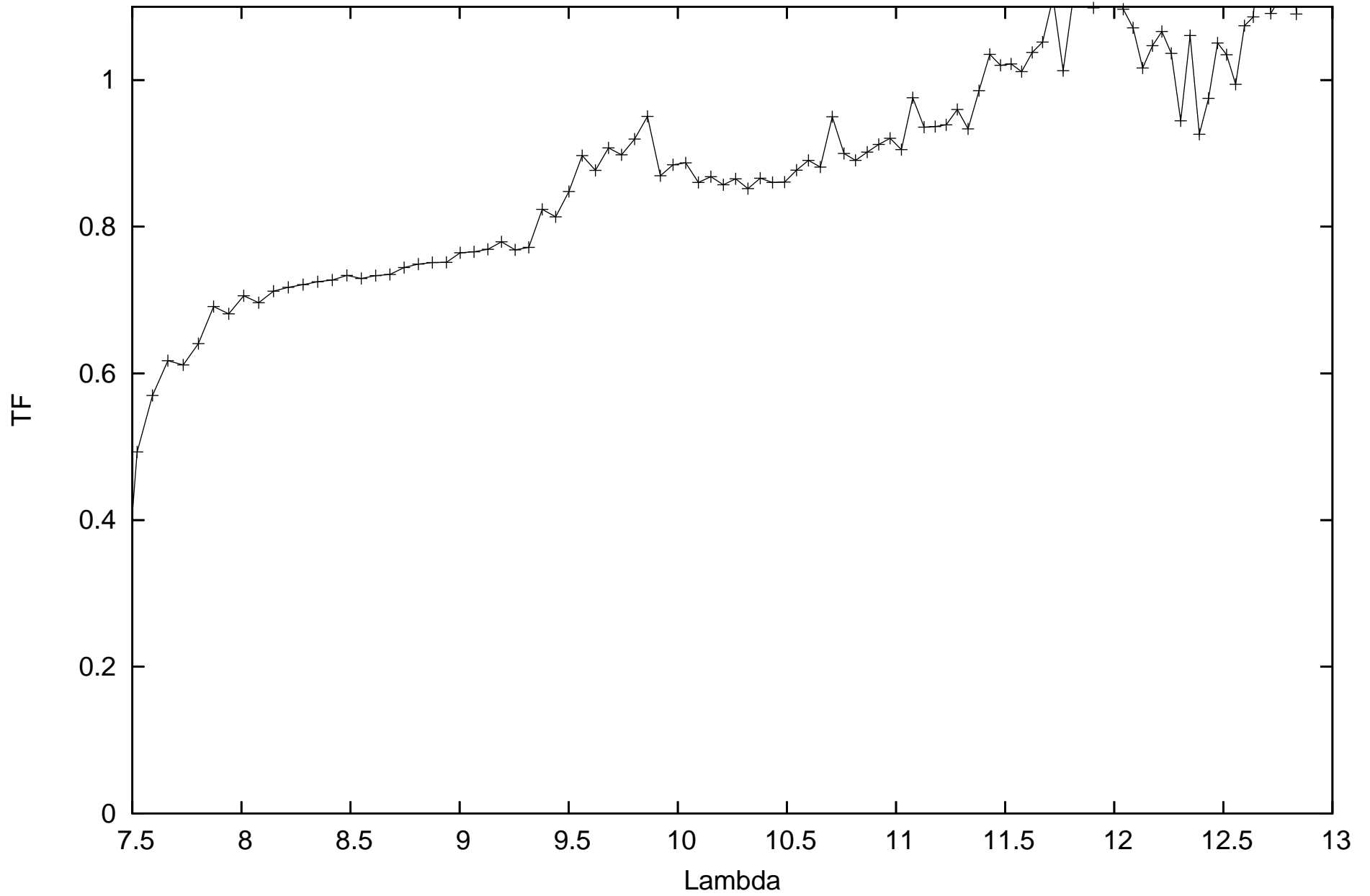
calHIP9884_flux-0.75397_diam7.42869_r.MIDI.2012-10-05T06_46_02.000_K0J3
