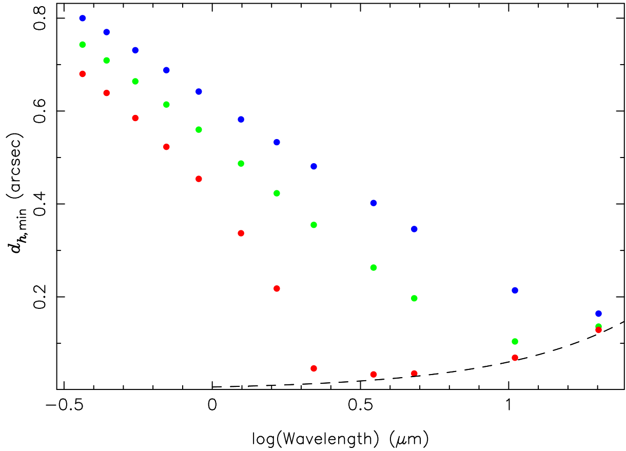
Fig. 1.— d_{h,\text{min}} = 50\% encircled energy diameter as a function of band, i.e. a graphical representation of Table 4. Blue = no AO, green = GLAO, red = LTAO. The dashed line shows the radius of the diffraction limited core of a perfect PSF for a D = 42 m telescope.
