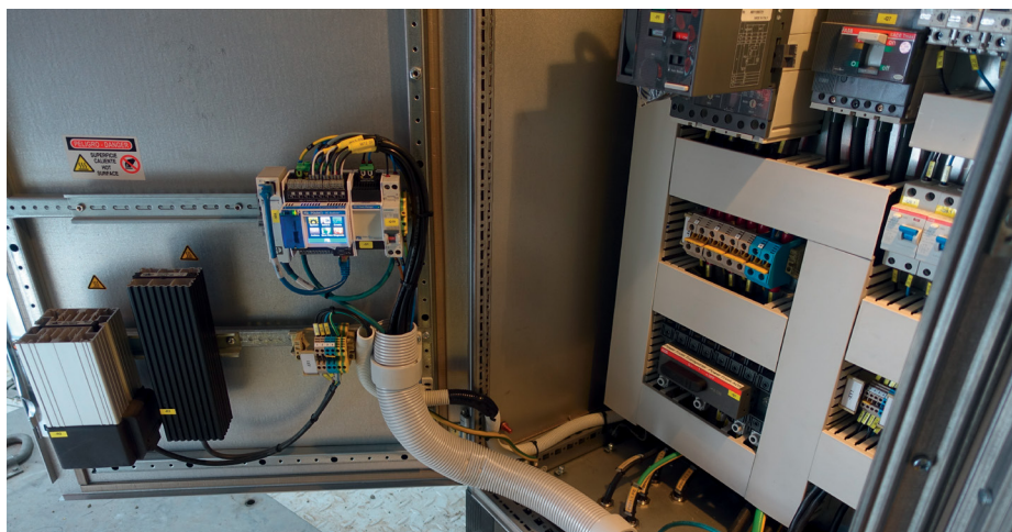
The Power Monitoring System installed in the pedestal of a European ALMA antenna.
