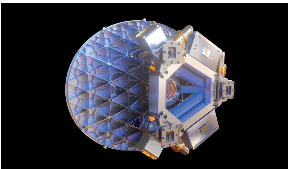
Rendering of the ELT's M5 mirror, a flat, fast tip-tilt mirror measuring 2.7 × 2.2 metres.
