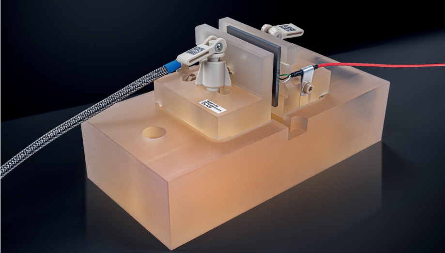
The ELT M1 edge sensors measure the relative positions of the ELT's primary mirror segments, allowing the overall shape of the mirror to be corrected when
