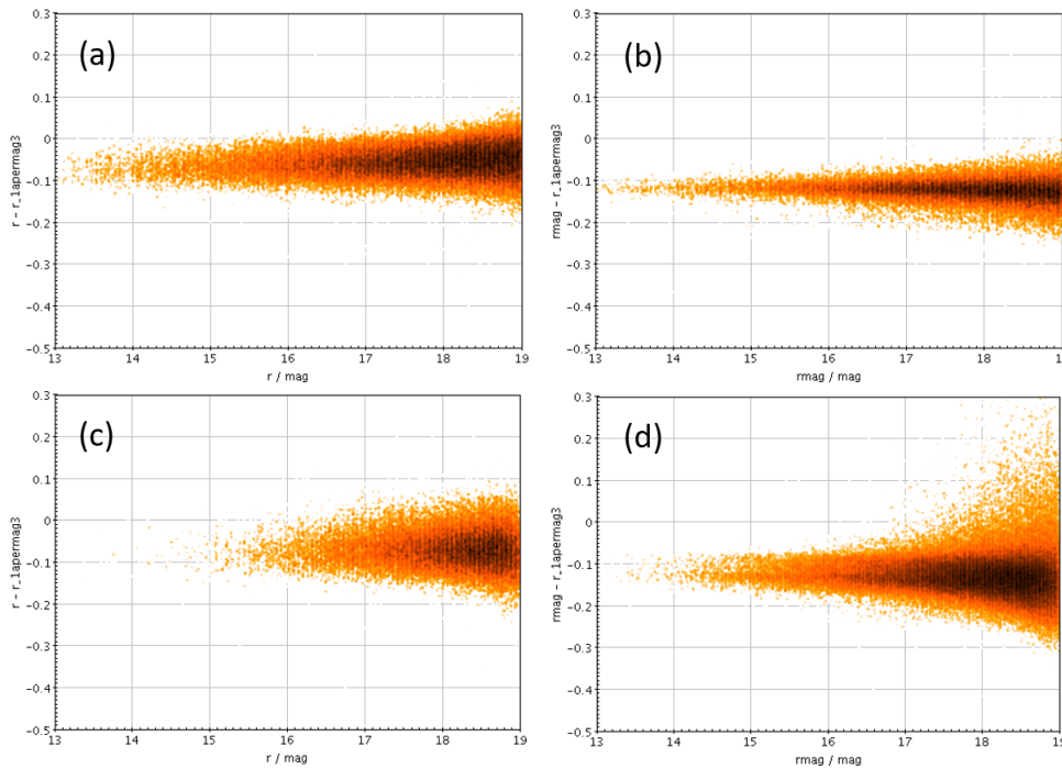
Figure 2: In the top row, r band magnitudes in the DR3 catalogue obtained from a 1-degree radius cone selection centered on l = 213^\circ , b = 0.0^\circ are compared directly with (a) IPHAS DR2 r ( A10POINT=1 ), (b) VPHAS+ DR2 r ( CLEAN=1 ). These are point-density plots such that the dark brown colour is associated with the highest point density, fading to white at lowest density. In all cases, the variable on the vertical axis is the difference between the AB DR3 magnitude and the Vega magnitude derived from IPHAS or VPHAS+ DR2 (as supplied by Vizier): the expected mean of this difference is -0.15 mags. Notice that the VPHAS+ DR2 and DR3 selections compared in panel (b) are based on the same VST observations – they differ in cross-matching strategy and method of photometric calibration. In these examples, the AB to Vega mean shifts illustrated differ by \sim 0.05 mags and neither is as negative as the recommended -0.15 . Panels (c) and (d) are analogous plots for a 1-degree radius cone selection at l = 33^\circ , b = 0.0^\circ at the opposite end of the VPHAS+ footprint, where source densities are typically several times higher and the influence of Southern-winter observing conditions is apparent. Again the mean AB-Vega offsets are different in (c) and (d), and there is evi-
