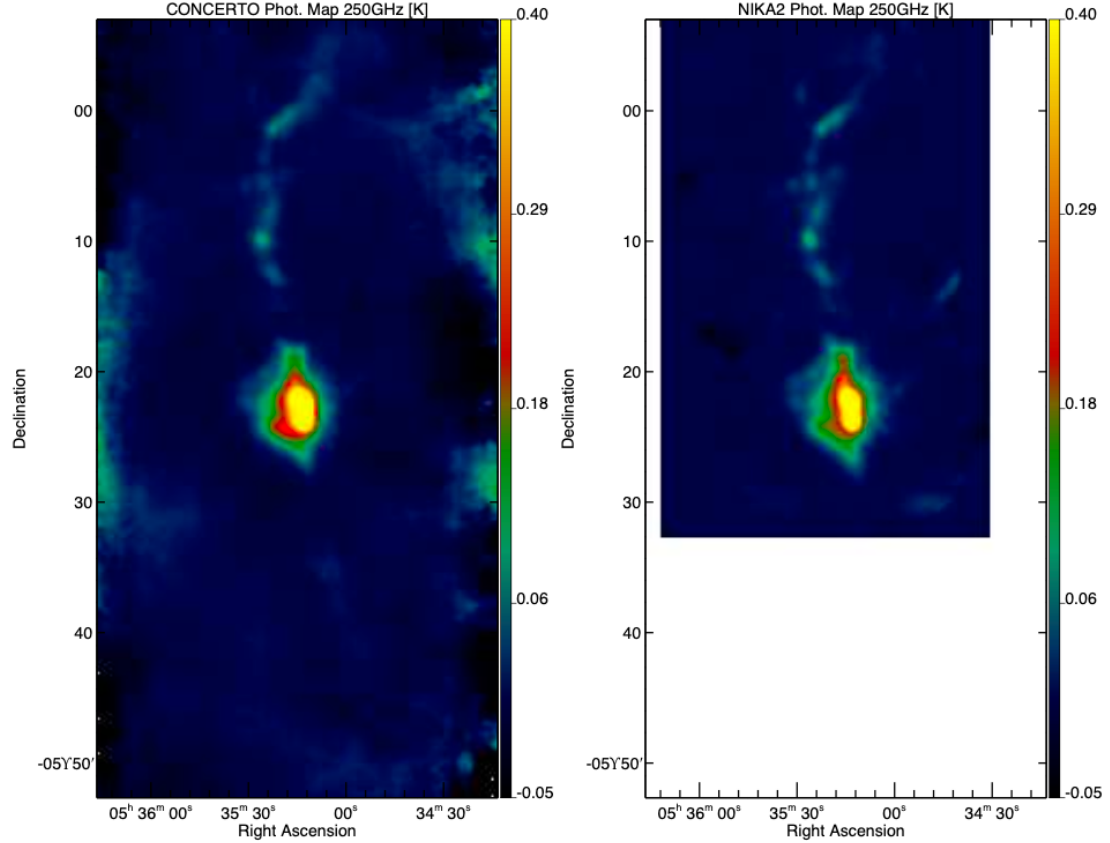
Fig. 2. Photometric map of Orion with CONCERTO (left) and NIKA2 (right) in brightness temperature at 250 GHz, convolved to a common 40'' resolution. The colour bar is in Kelvin, and the maps are saturated at 0.4 K to highlight faint structures. Both instruments recover the same large-scale morphology and diffuse emission. A direct pixel-by-pixel comparison (not shown here, see Désert et al. 2025, Fig. 3) demonstrates a tight linear correlation with unit slope, confirming that CONCERTO’s calibration is consistent with NIKA2 to within \sim 15\% . This establishes the reliability of CONCERTO photometry across extended emission regions, while providing the unique advantage of simultaneous spectral coverage from 130 to 310 GHz.
