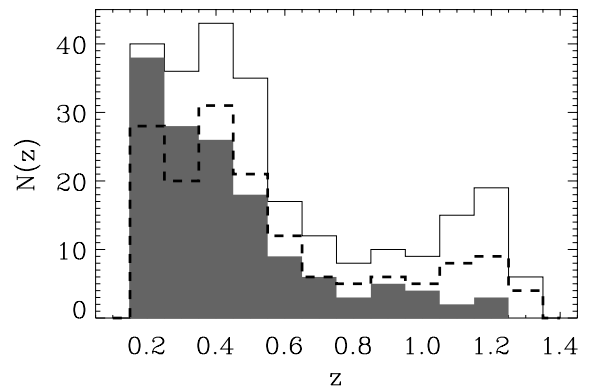
Fig. 2. The redshift distribution for the cluster candidates detected in Patches C and D. The shaded area marks the distribution for the “good” candidates as defined in the text. The dashed line shows the distribution for the candidates detected in the paired catalogs
