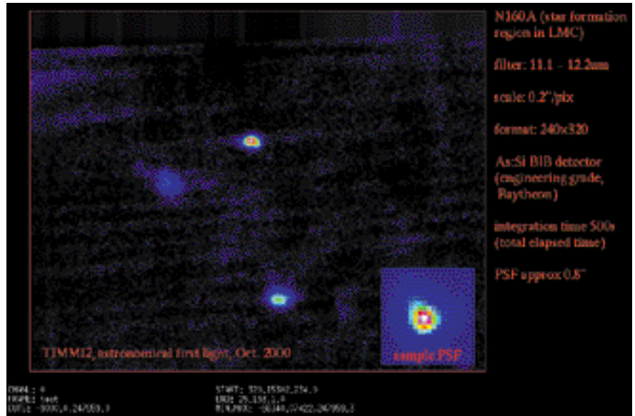
Figure 5: Image of the LMC star-formation region N160A. This was one of the first integrations on a scientifically interesting target with TIMMI2. The residual stripiness is due to grounding problems. While in principle this could be easily removed by Fourier filtering of the data, the cause is understood and the ground-loop problem will be solved while this article goes into print. The insert shows at a magnified scale a typical point-spread-function.
