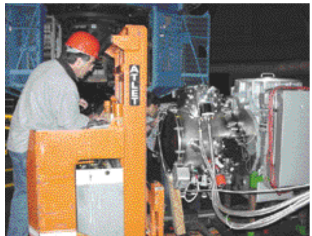
Figure 4: The TIMMI2-adapter assembly on its way to the telescope. While TIMMI2 could be hand-carried conveniently to the telescope, TIMMI2 needs a fork-lift and other special tools. The metal hoses lead to the closed-cycle cooler expansion machine attached to the top of the vacuum vessel. The TIMMI2 cryostat is interfaced to the recycled f135 adapter by means of a special alignment plate which holds also a wheel with calibration targets.
