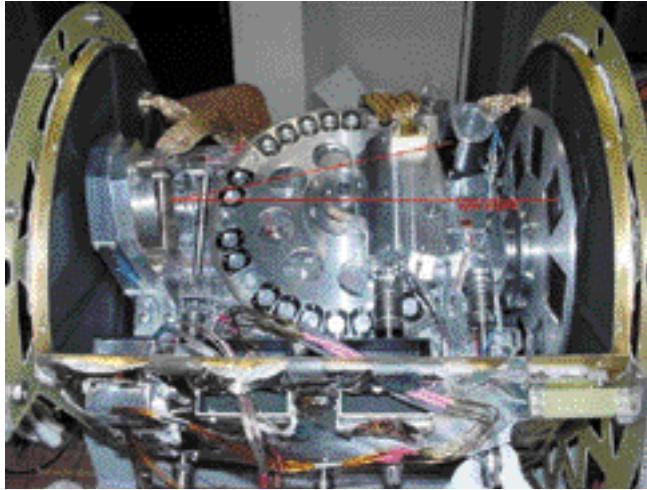
Figure 3: Close view from the top of the TIMMI2 cold optical bench (baffles and shields partially removed). Left and right in the picture the fibre-glass support structure and the solid parts of the radiation shield can be seen. To guide the eye, the optical path, starting on the right at the aperture/slit-wheel leading to the collimator and from there to the folding mirror is indicated. The folding mirror sends the light through the (encapsulated) polariser unit to the filter wheel, cold stop and lens wheel, then to the detector unit which is mounted to the back of the bench. The distance aperture/slit wheel to collimator is \approx 350 mm. Three drive shafts are clearly visible, from left to right: filter-wheel, polariser movement and polariser insertion.
