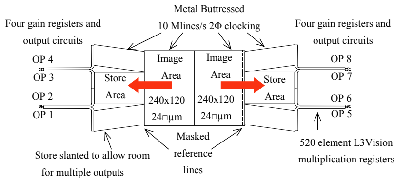
Figure 1. Schematic of CCD220.
