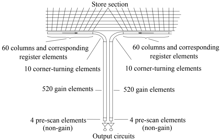
Figure 2. Details of serial and gain register.
