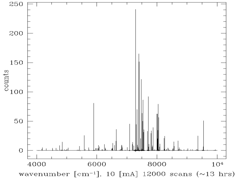
Figure 2: Near-IR spectrum of a Th-Ar hollow cathode lamp taken with ESO's FTS
