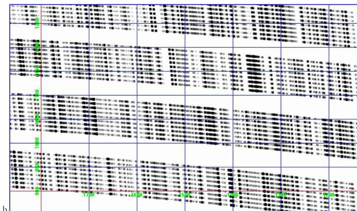
Figure 3. a. Section of a real 9 pin hole mask, Th-Ar HCL exposure. b. Equivalent section of a physical model simulation based on the fitted model parameter set
