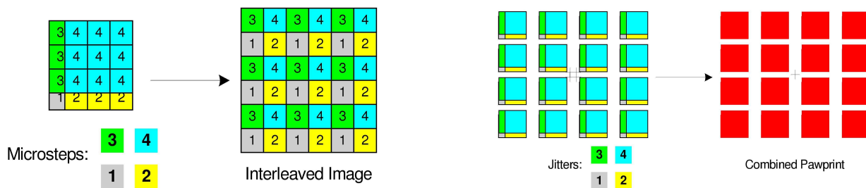
Figure 12: Combining exposures with microstepping (left) and jittering (right). Each numbered square corresponds to one pixel.
