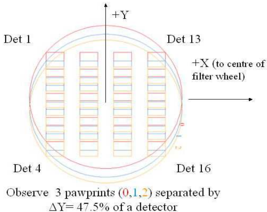
Figure 14: Completing a tile with six pawprints: the three vertical steps along the Y axis.
