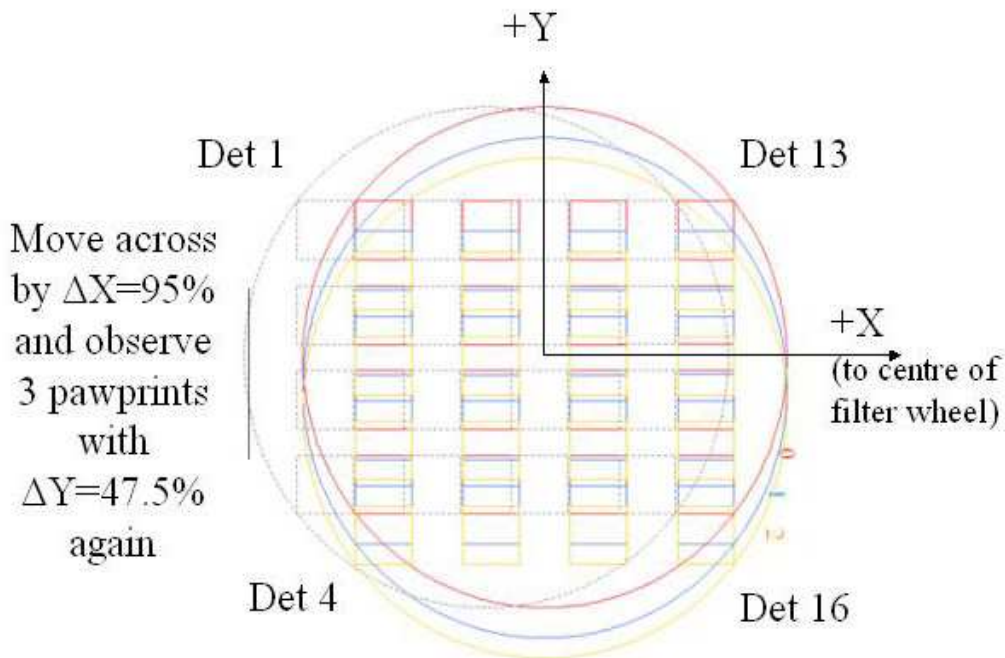
Figure 15: Completing a tile with six pawprints: the two horizontal steps along the X axis.
