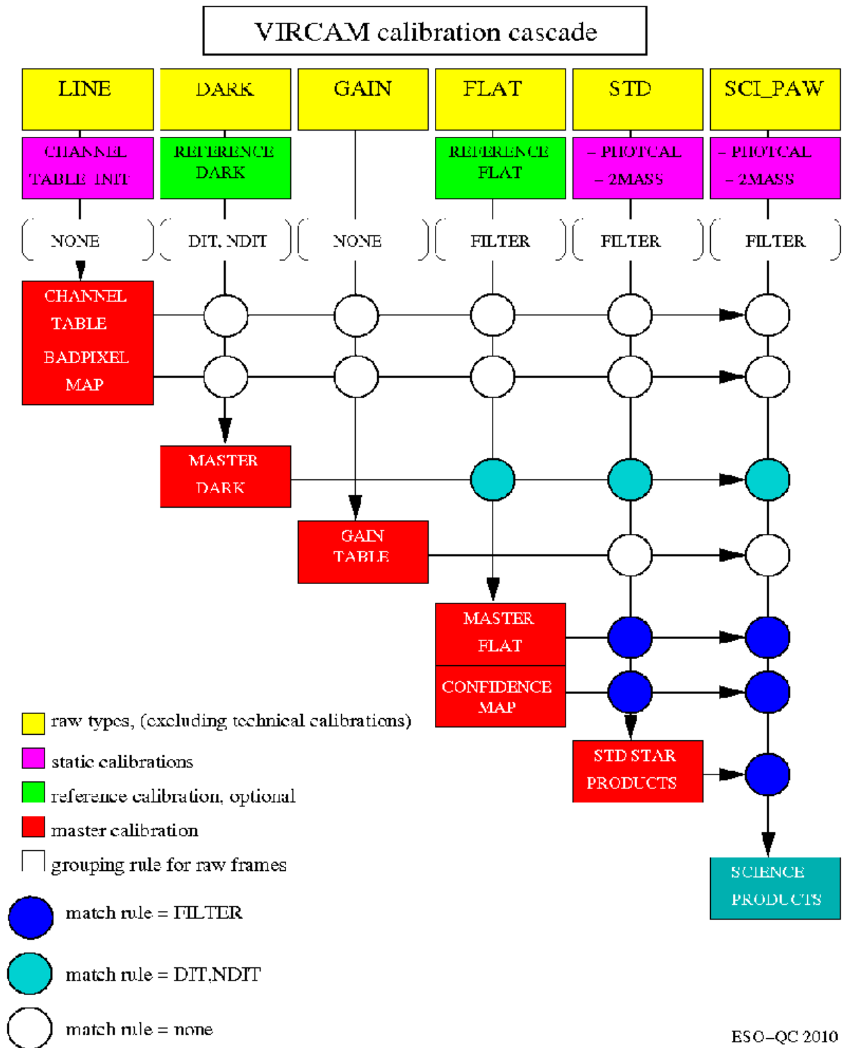
Figure 22: VIRCAM cascade diagram for producing calibration frames.
