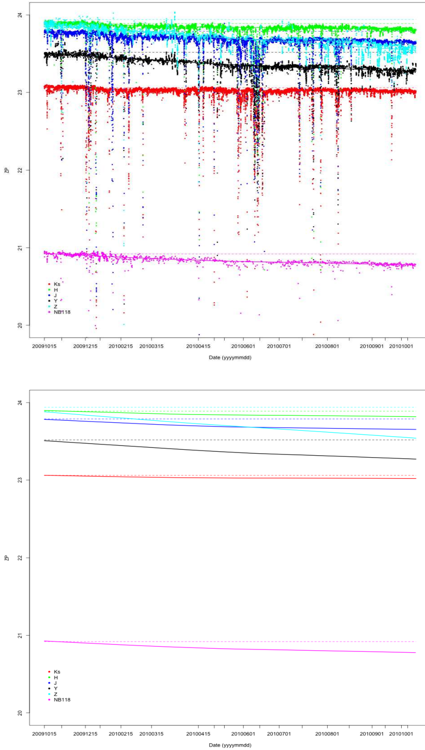
Figure 10: Zero point trends during the first year of operation 2009-2010. Courtesy of CASU.
