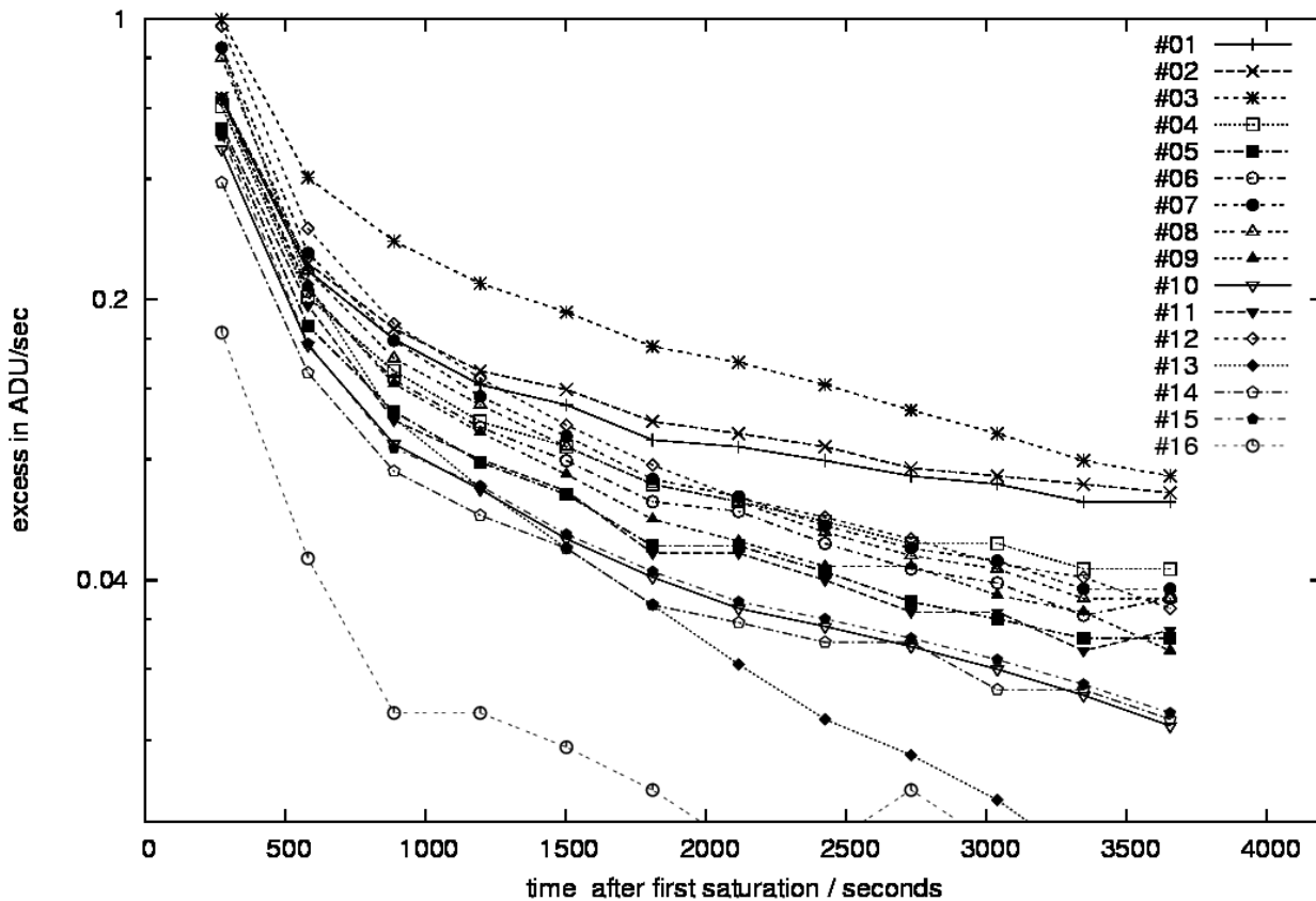
Figure 7: VIRCAM persistence for the individual detectors.
