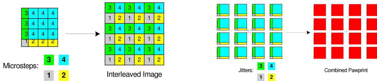
Figure 15: Combining exposures with microstepping (left) and jittering (right). Each numbered square corresponds to one pixel.
