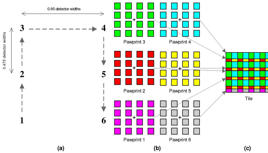
Figure 19: Contiguous tile, formed by combination of six overlapping pawprints.
