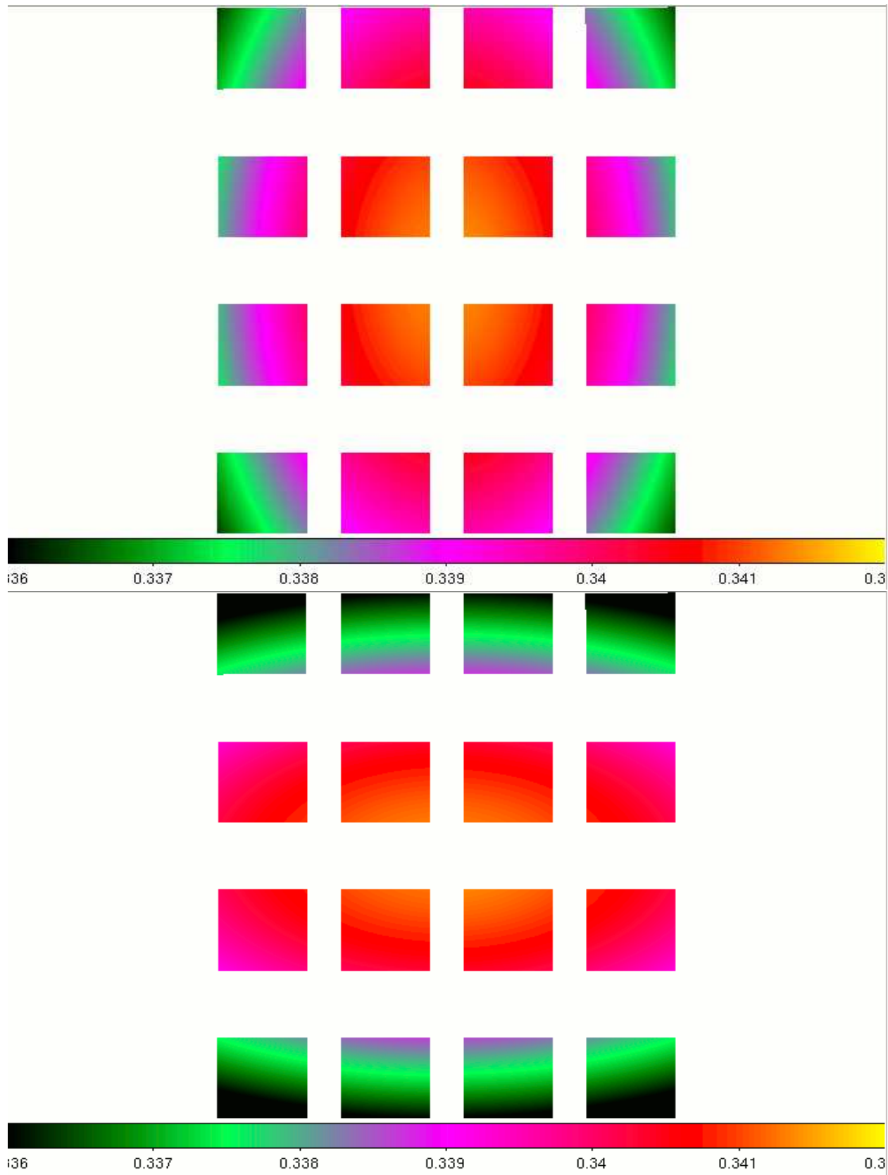
Figure 24: Maps of the pixel sizes across the focal plane, along the X (top) and Y (bottom) axis. Based on data from 2009-01-26.
