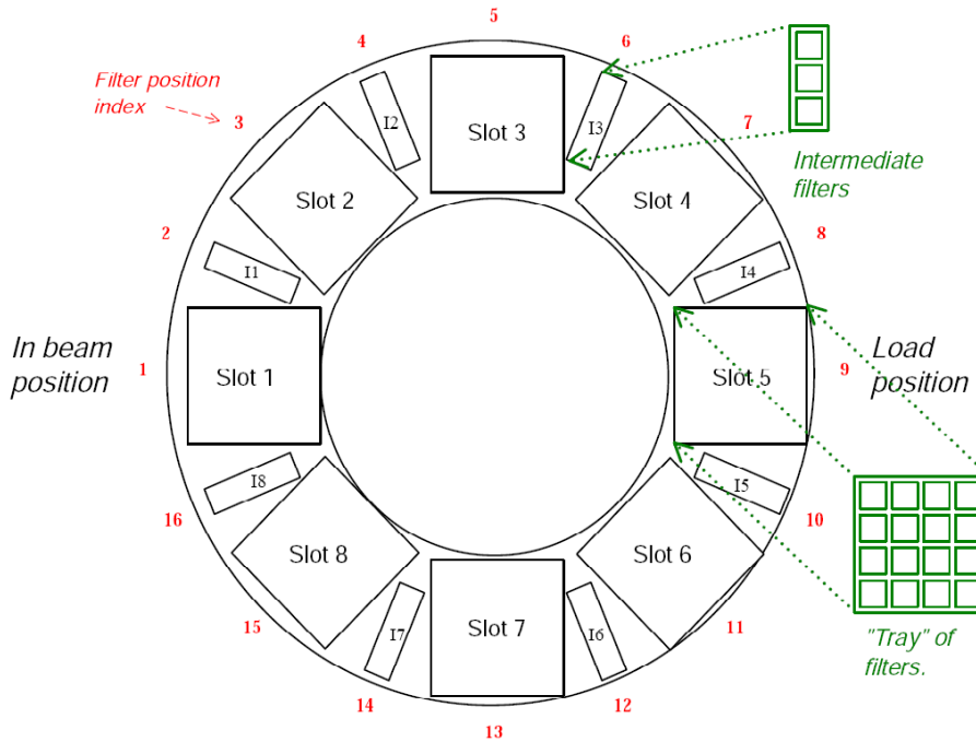
Figure 9: Layout of the VIRCAM filter wheel.
