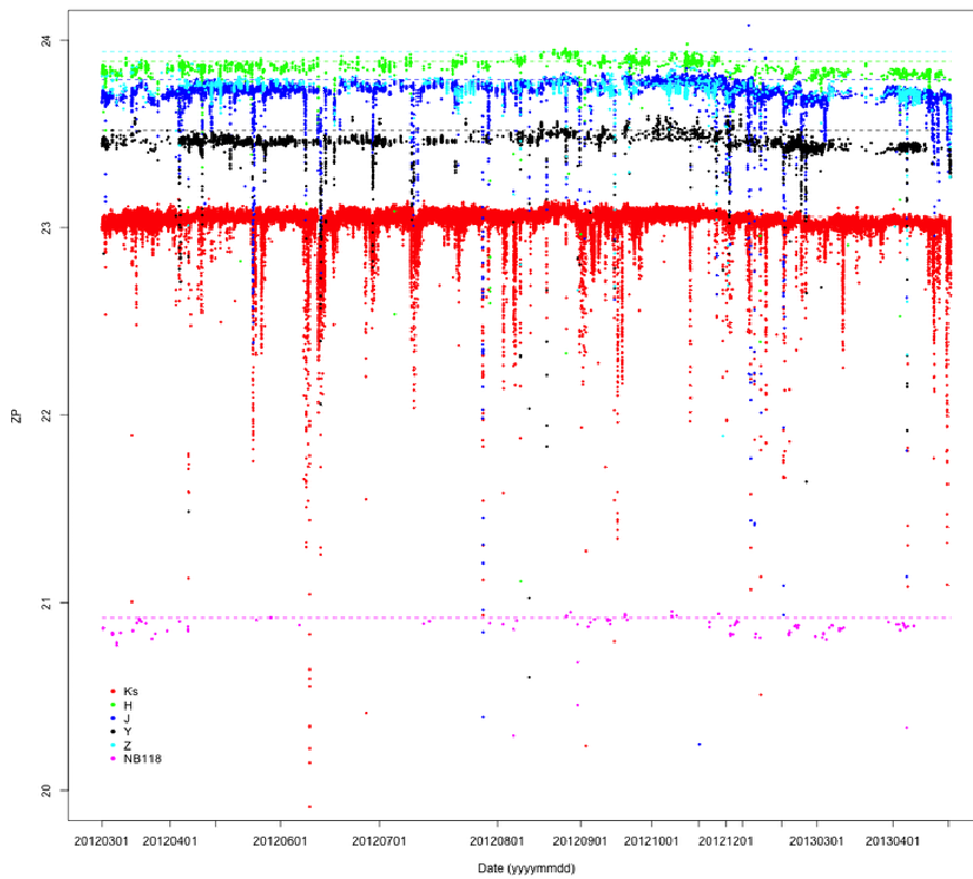
Figure 13: Zero point trends in 2012–2013. Courtesy of CASU.
