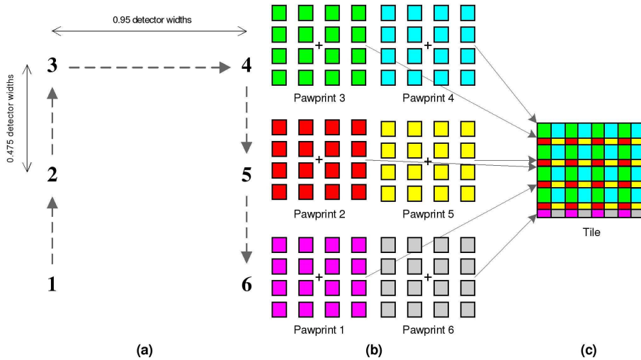
Figure 19: Contiguous tile, formed by combination of six overlapping pawprints.
