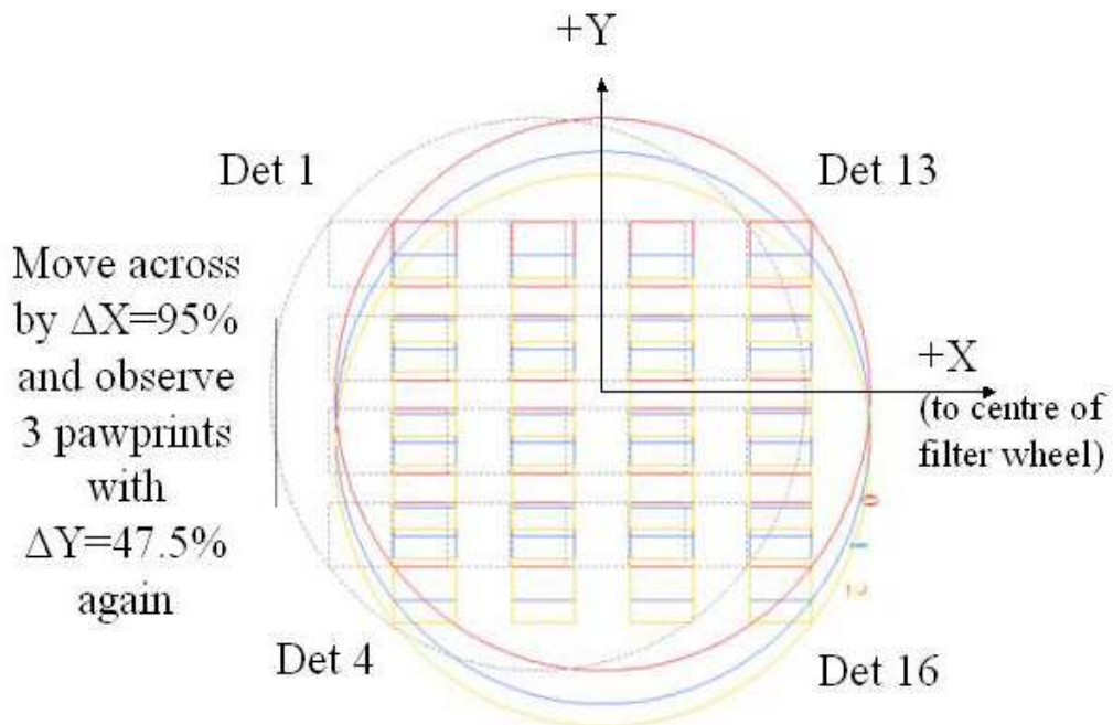
Figure 18: Completing a tile with six pawprints: the two horizontal steps along the X axis.
