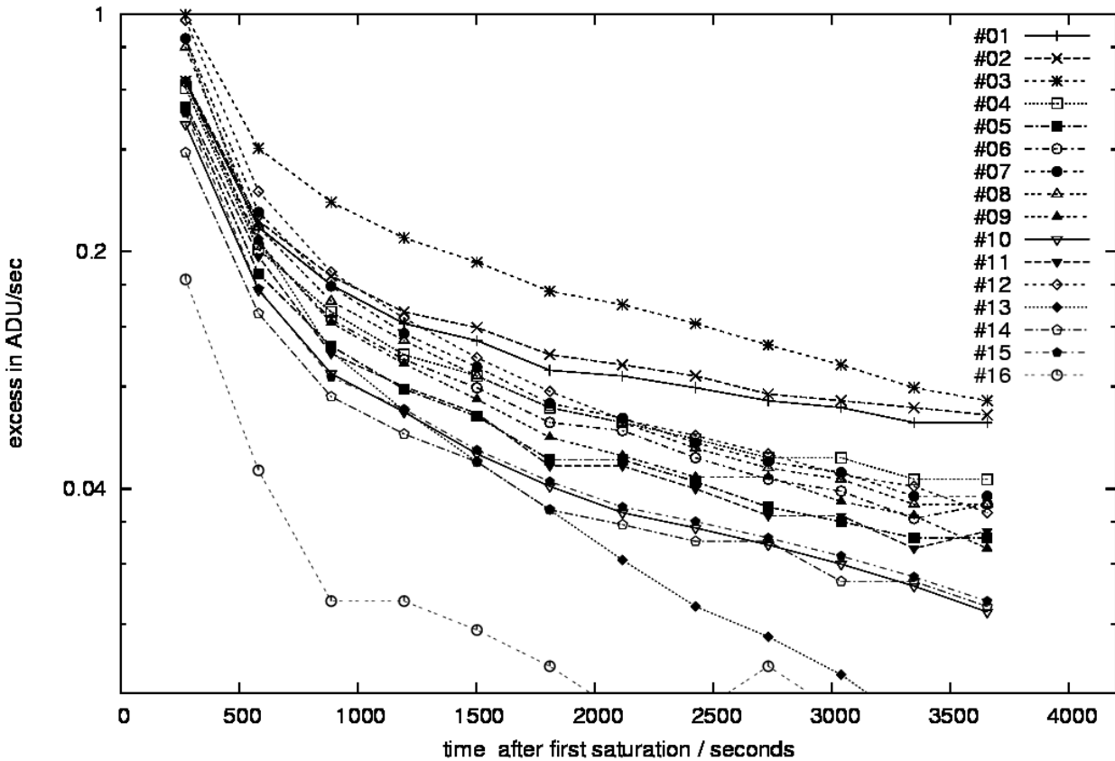
Figure 7: VIRCAM persistence for the individual detectors.
