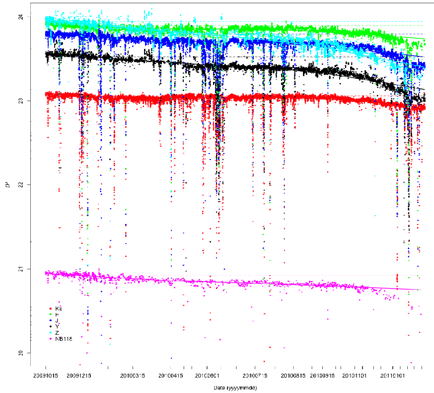
Figure 11: Zero point trends in 2010–2011. Courtesy of CASU.
