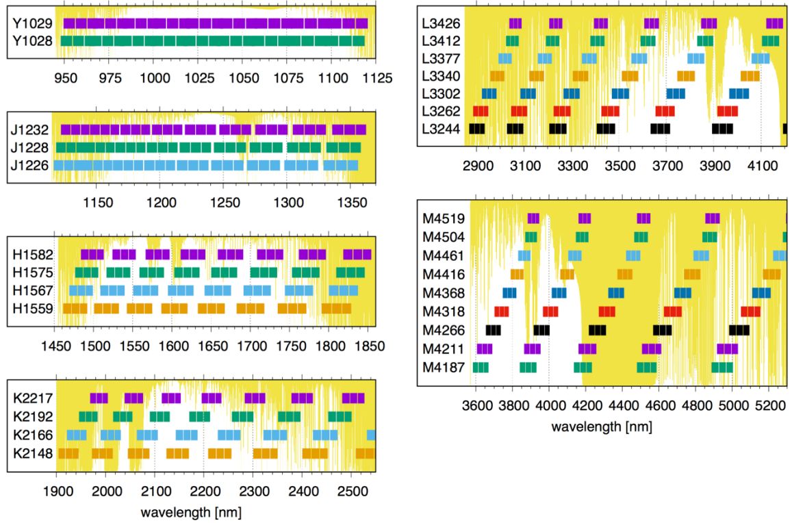
Figure 39: CRIRES wavelength settings compared to the atmospheric transmission. 4
