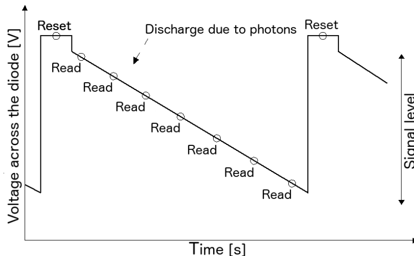
Figure 24: “Sample Up The Ramp” read-out mode. Before each integration, the pixels are reset to the initial capacity. During the integration, the detector is non-destructively read (from two readings in case of the minimum DIT up to a maximum of 36 readings for long DITs). These detector readings are equidistantly spaced in time. The flux rate per pixel corresponds to the slope of the flux values of the subsequent readings.
