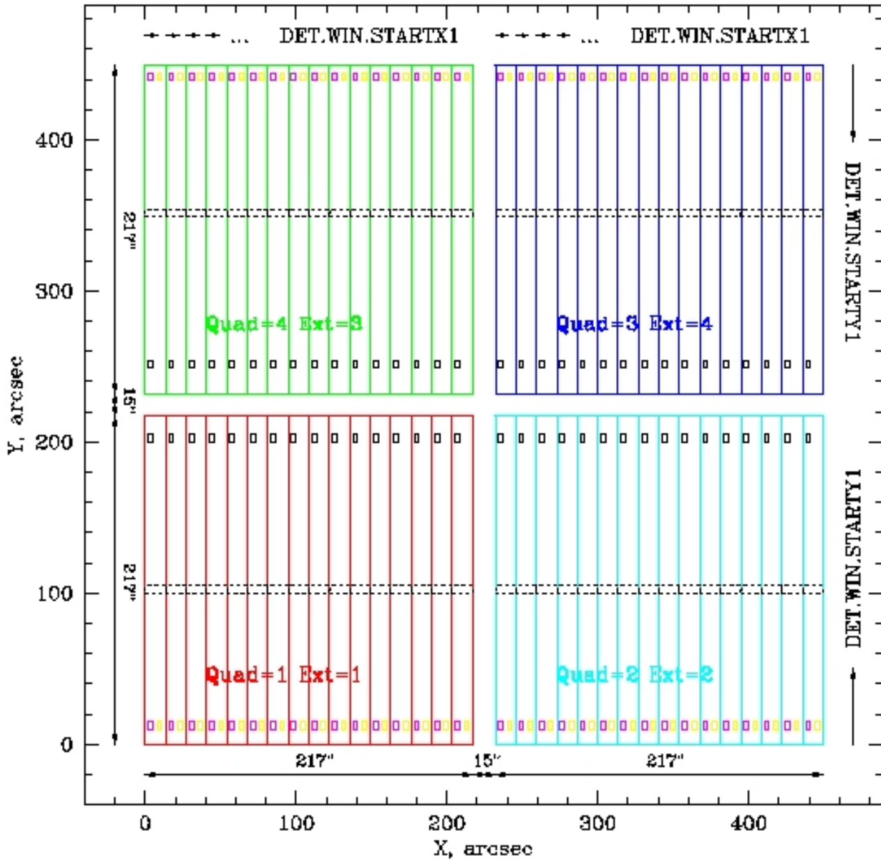
Figure 12: Definition of the windows. The location of the four HAWK-I detectors on the focal plane are shown, as well as the 16 stripes in which each detector is being read. The sizes of the detectors and the gaps, projected on the sky in arcsec are also given. The binaries generated from quadrants 1, 2, 3, and 4 are usually (but not always) stored in fits extensions 1, 2, 4, and 3. Arrows indicate the direction in which the parameters DET.WIN.STARTX, DET.WIN.STARTY, DET.WIN.NX and DET.WIN.NY increase. Note, that the parameter DET.WIN.STARTX defines the starting point of the window, counted from the beginning of each detector stripe, not from the beginning of the detector. Note that all these parameters are defined in pixels, although this figure is plotted in arcsec. Four different sets of windows are shown in violet, yellow, solid and dashed black lines.
