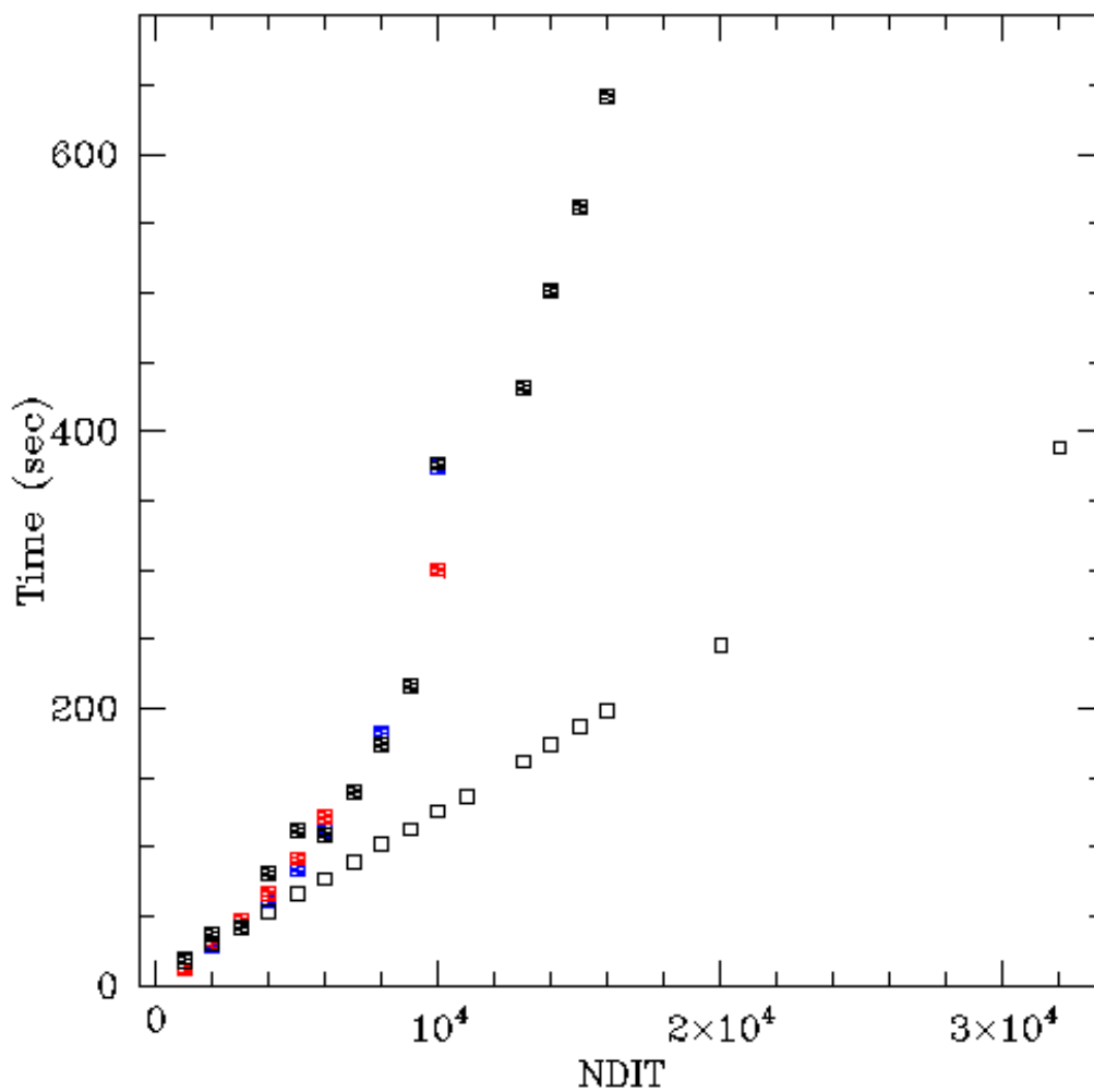
Figure 7: Execution times of the ISAAC LOW .img_acq.FastPhot template depending on the the data cube size and the selected mode (Burst or FastJitter). Filled squares are for Burst mode executions (black is for window=32x32 and DIT=3.2ms; blue is for window=32x32 and DIT=5ms; red is for window=64x64 and DIT=6.4ms). Empty squares are for the FastJitter mode executions (window=32x32 and DIT=12 ms).
